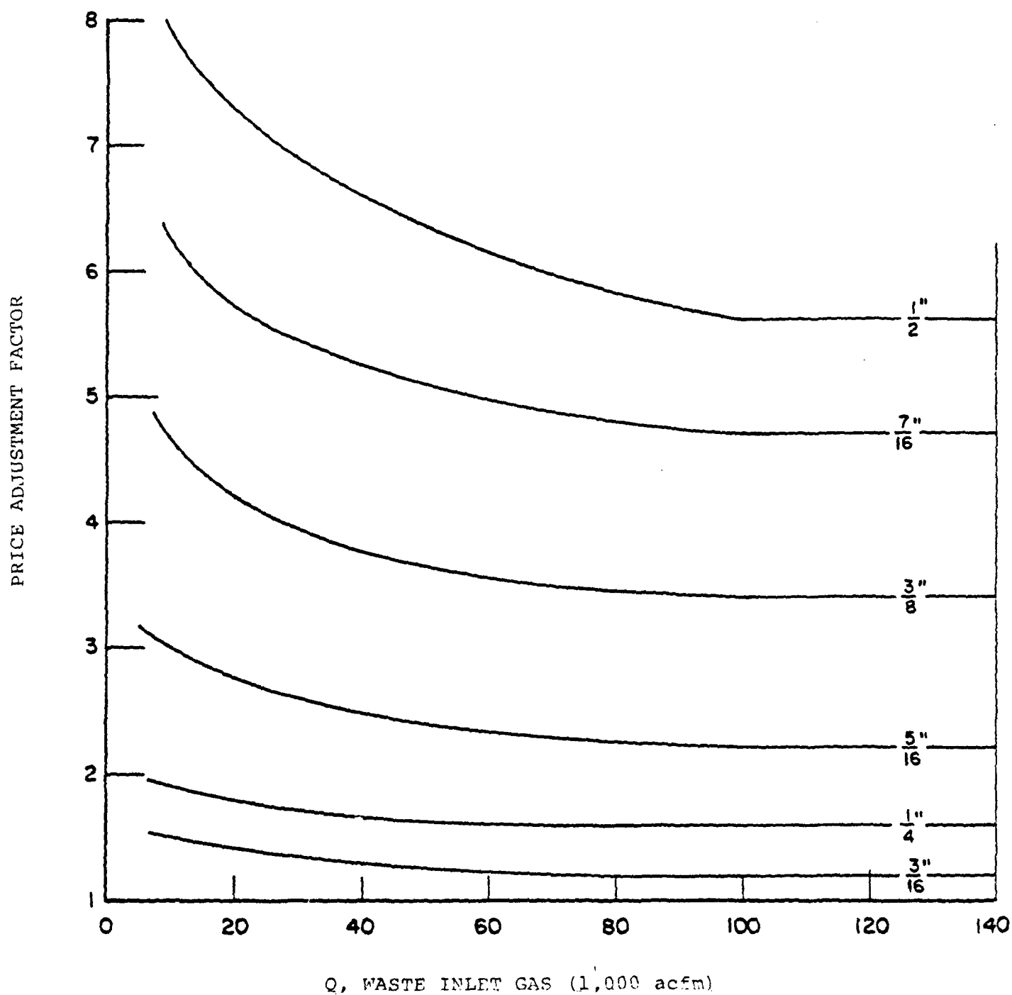
FIGURE 4-2 PRICE ADJUSTMENT FACTORS VS. PLATE THICKNESS AND VOLUME 35
