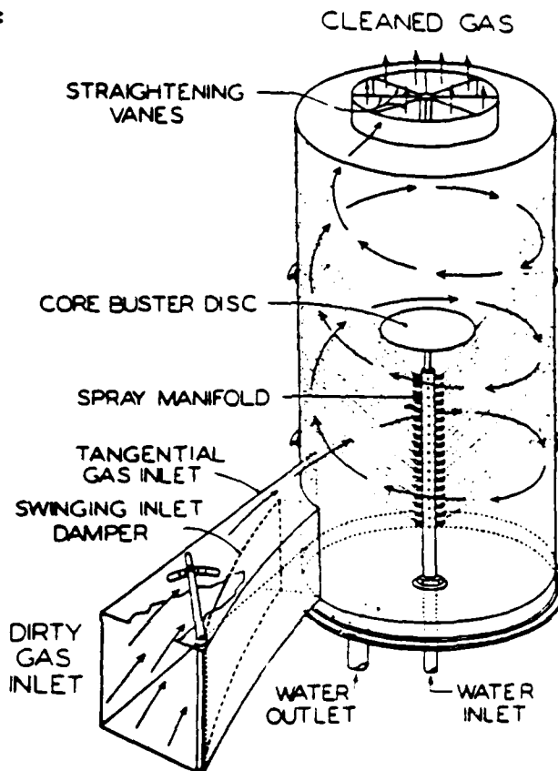
Cyclonic Spray Chamber
