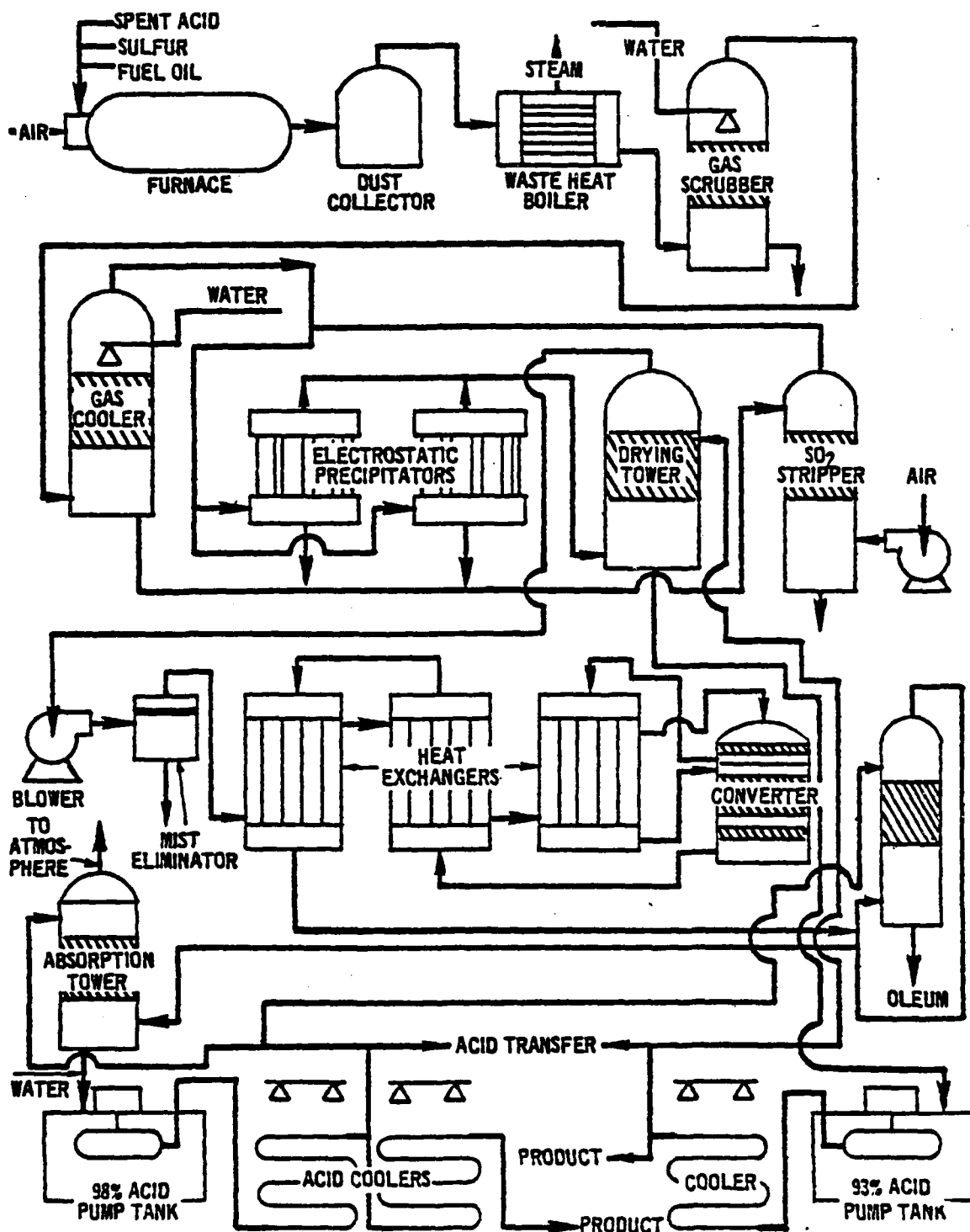
FIGURE 1-12 BASIC FLOW DIAGRAM OF CONTACT-PROCESS SULFURIC ACID PLANT BURNING SPENT ACID 17
