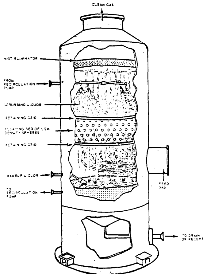
Moving Bed Scrubber
