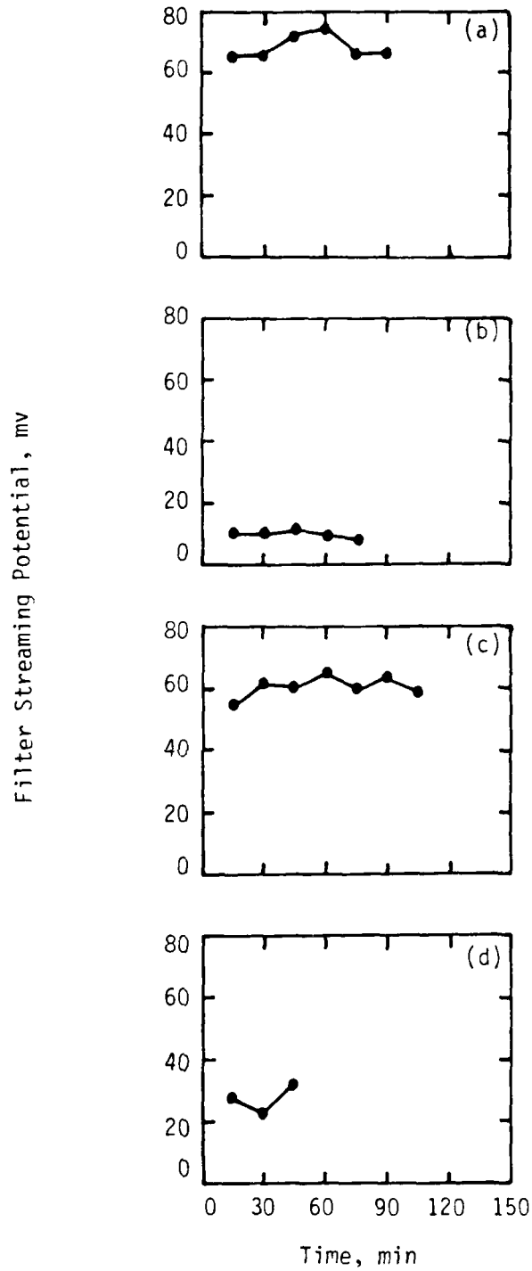
Figure D7 Filter streaming potential readings vs. time. Des Plaines River (Influent Turbidity = 35 FTU). Polyelectrolyte Dosages: (a) 0 mg/l, (b) 0.5 mg/l, (c) 1.0 mg/l, (d) 1.5 mg/l.
