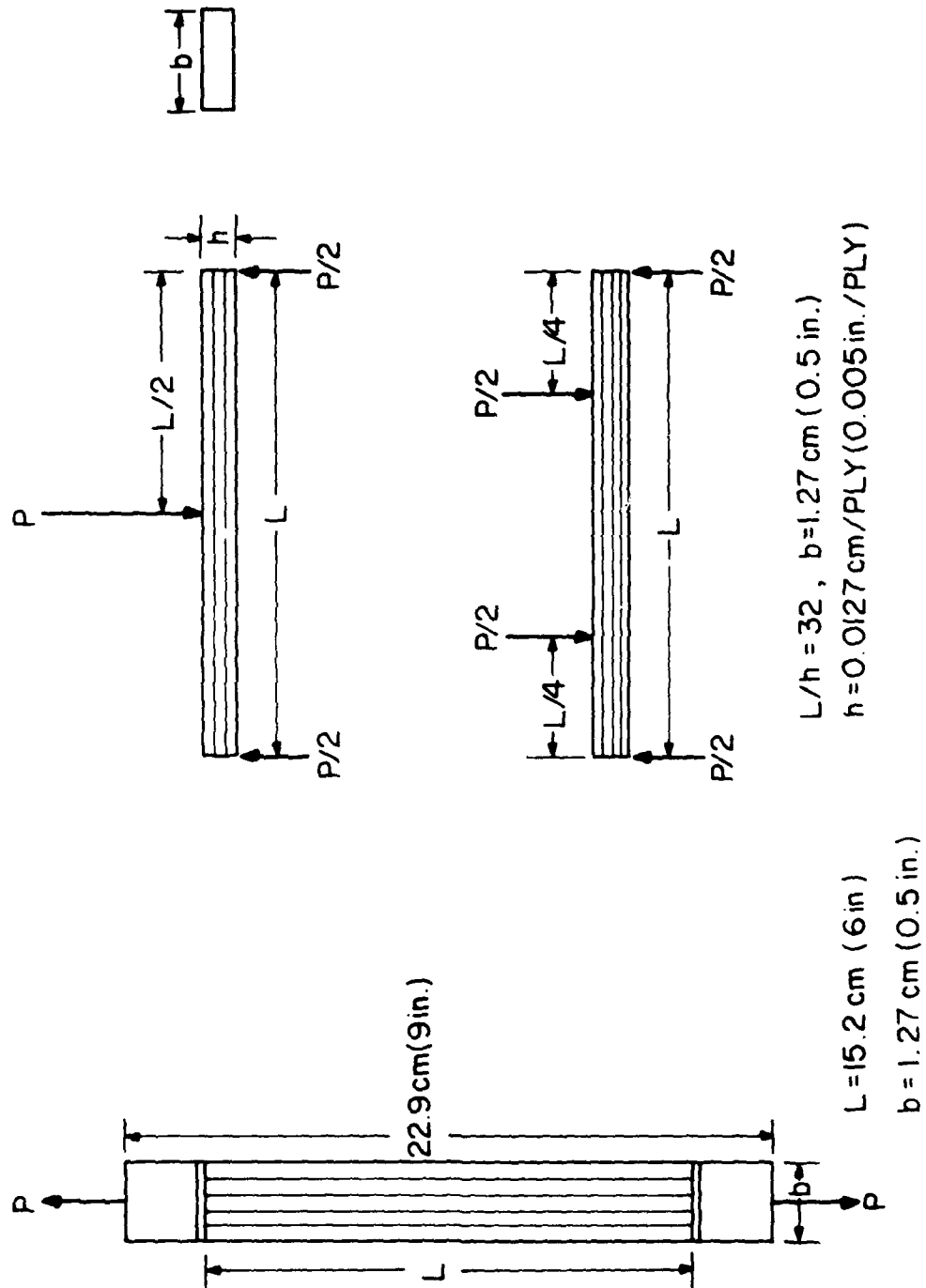
Figure 1. Geometry of Test Specimens.
