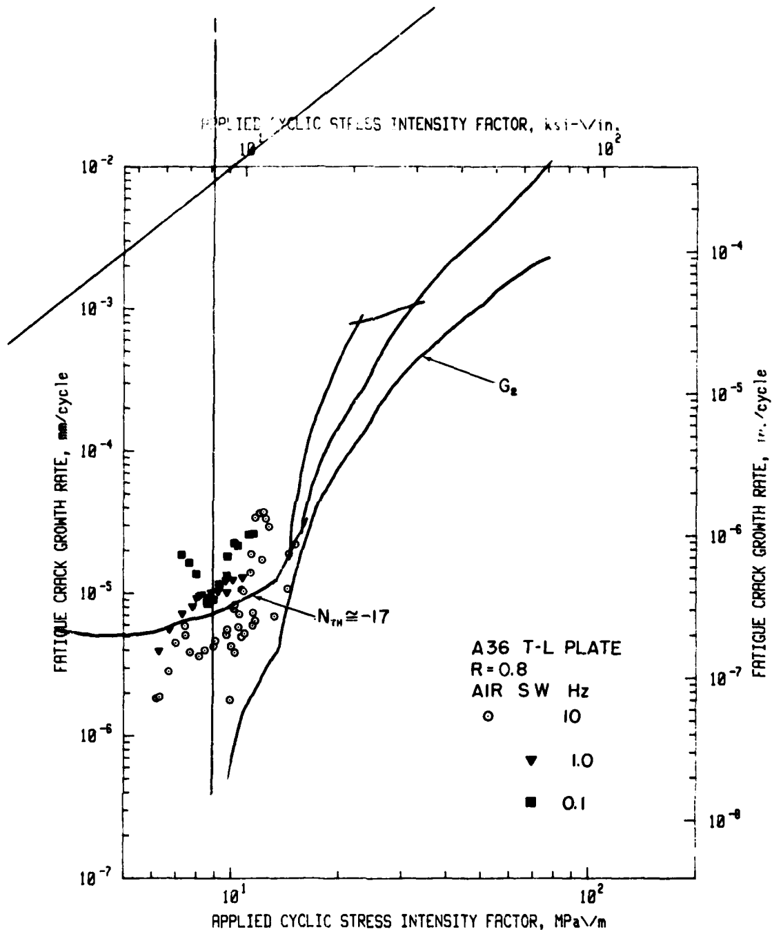
Fig. 18 - Parametric curves from Fig. 14, are shown in match at d_T = 8 . Fig. 13. \mu m to composite data for R = 0.8 , Fig. 13. The "constant N " curve members in the threshold region are of same indexes as for the R = 0 data of Figs. 16 and 17.
