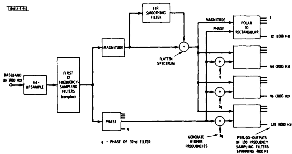
Fig. 14. Method for generating excitation spectrum from baseband.
