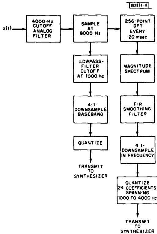
Fig. 13. Proposed structure for analyzer of possible baseband-excited vocoder.
