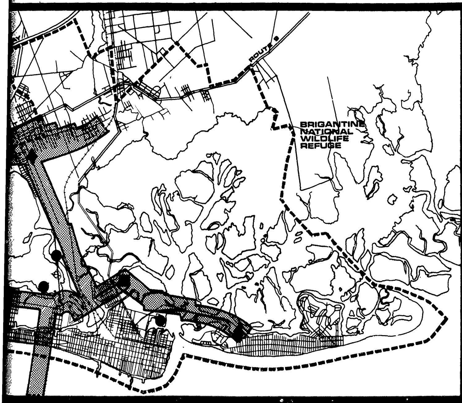
THE ATLANTIC COASTAL REGION SEWERAGE SYSTEM
