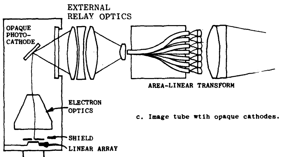
Figure 31. Electron bombardment coupled.
