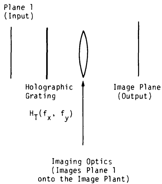
Figure 2-5. Position Invariant Property of Frequency Domain Filtering System
