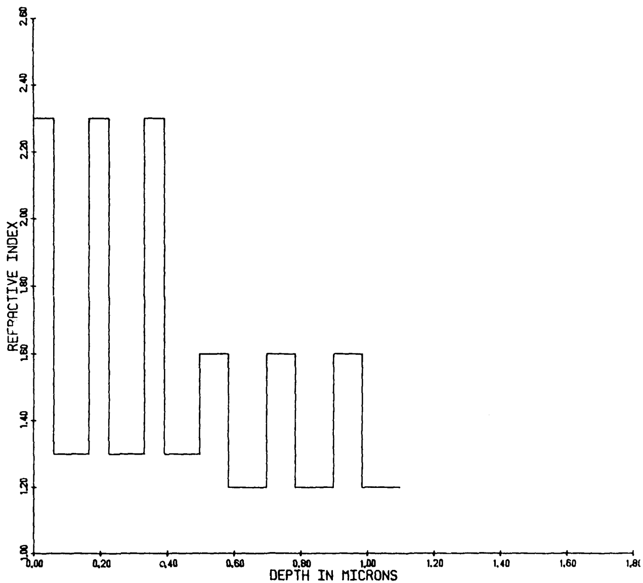
Figure 3-2. Twelve Layer High-Low High-Low Dielectric Stack
