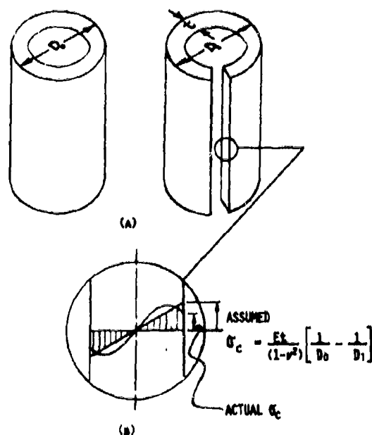
FIGURE 1. CRAMPTON'S METHOD FOR COMPUTING THE CIRCUMFERENTIAL STRESS IN THIN WALL TUBES.
