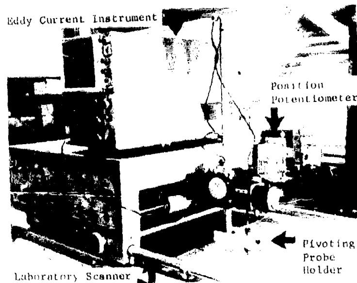
Figure 8. Eddy Current Scanning Apparatus
