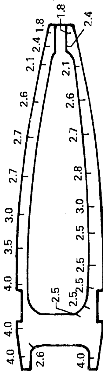
CIRCUMFERENTIAL CRACKS
