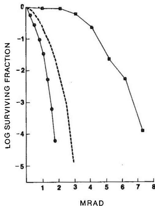
Figure 2. Comparative radiation resistance of M. radiodurans in beef. Symbols: ■, -30 \pm 10^{\circ}\text{C} ; ●, 30 \pm 10^{\circ}\text{C} . Broken line is replotted for M. radiodurans in beef puree at 5^{\circ}\text{C} (Fig. 1, Duggan et al., 1963a).
