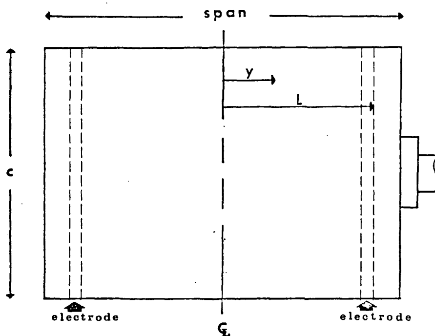
Figure 18. Placement of tencs sheet and copper strips (electrodes) on the test blade.
