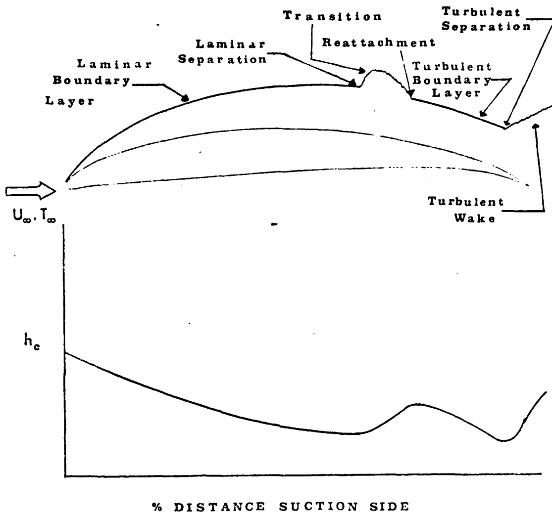
Figure 7. Schematic of a compressor blade in supercritical flow with the resulting convection heat transfer coefficient distribution.
