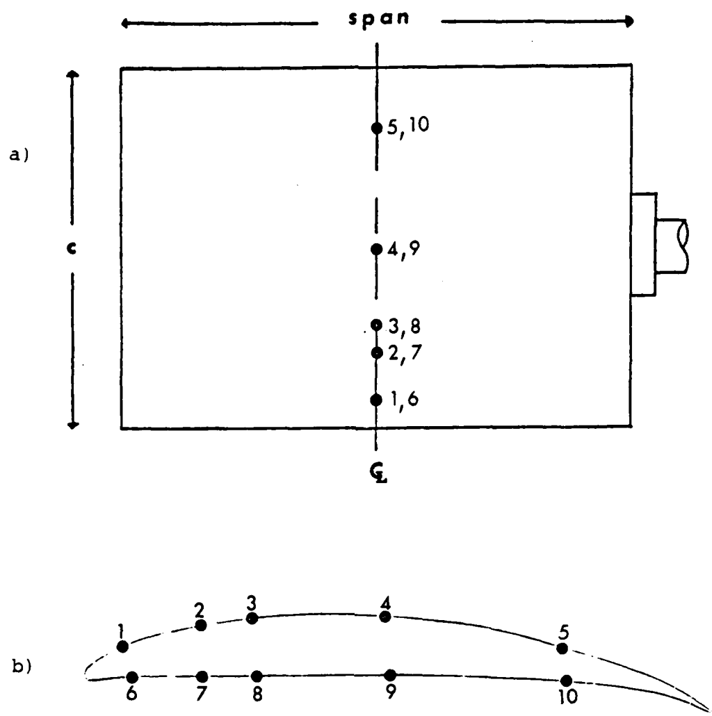
Figure 1. NACA 65 test blade showing location of thermocouples, a) top view, b) side view.
