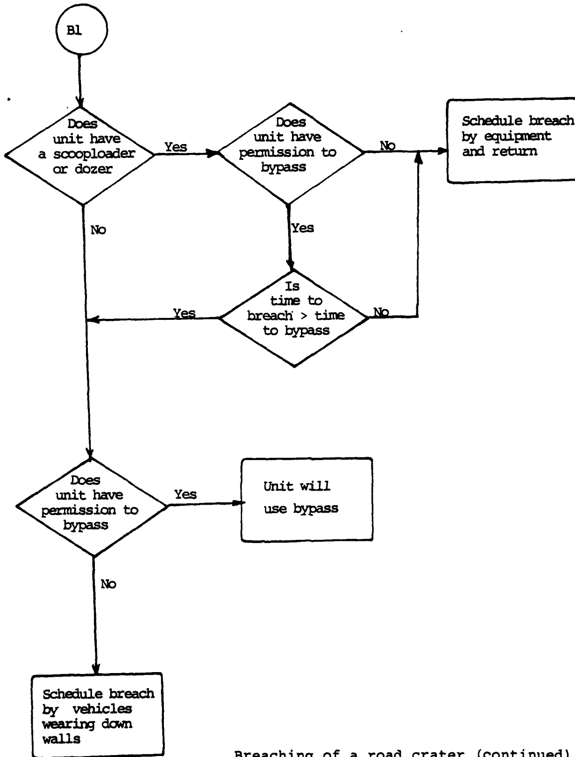
Breaching of a road crater (continued)
