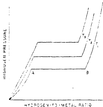
FIGURE 3.8 IDEALIZED HYDRIDE SYSTEM
