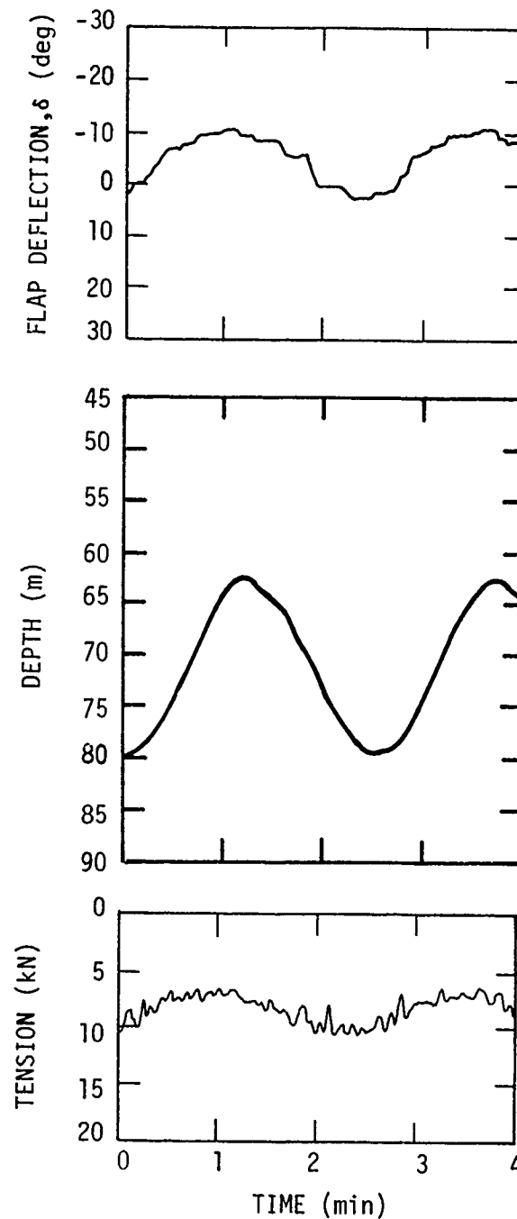
Figure 15b - Frequency, 0.0067 Hertz; Amplitude, Half Run (Run 27)
