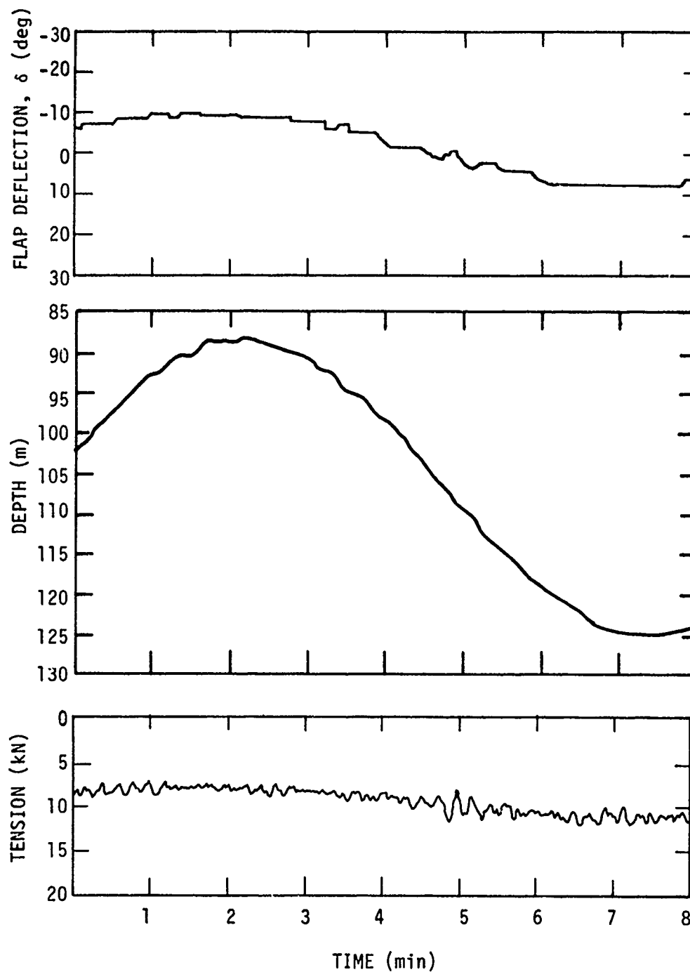
Figure 12a - Frequency, 0.0016 Hertz; Amplitude, Full (Run 13)
