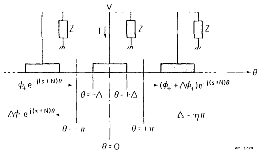
Fig. 11. Same as Figure 10 with dimensionless variables.
