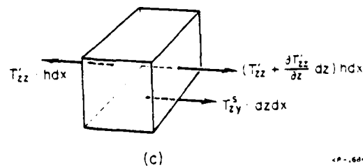
Fig. 2. First-order forces acting on a differential element of the strip in
