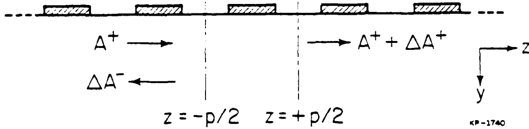
Fig. 7. Surface wave scattering from a single strip in a periodic array.
