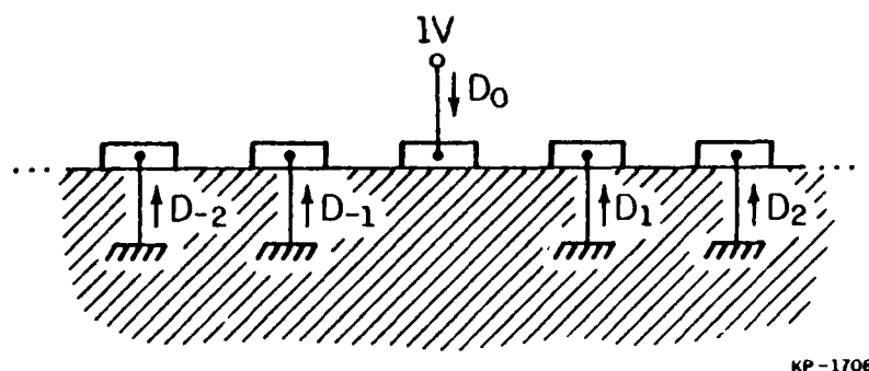
Fig. 15. Electrode currents in a single tap transducer.
