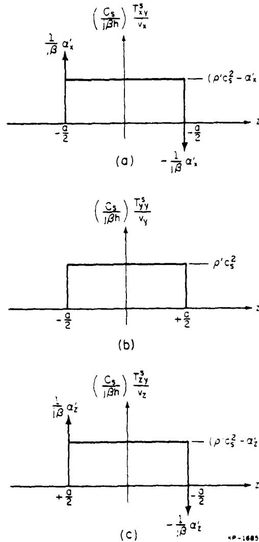
Fig. 3. Spatial distribution of (a) x-directed, (b) y-directed, and (c) z-directed interface stresses.
