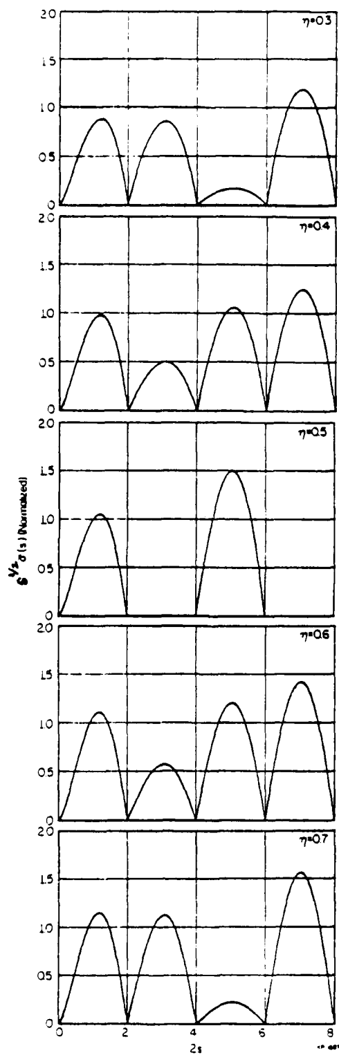
Fig. 16. Element factor for different metallization ratios.
