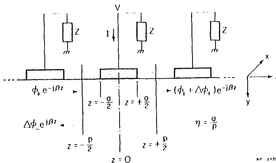
Fig. 10. Reflection and transmission of surface acoustic waves at an electrode in a periodic array.
