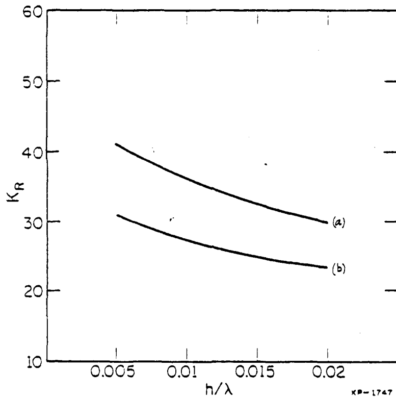
Fig. 9. K_R vs h/\lambda at the second harmonic for, (a) Grooves in ST-cut quartz (b) Aluminum electrodes on ST-cut quartz.
