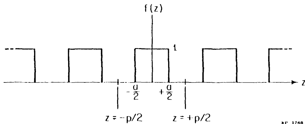
Fig. A2. Function describing geometry of the strips.
