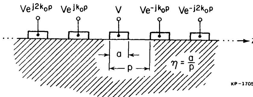
Fig. 13. A phased array transducer with a uniform phase progression of k_0 p per period.
