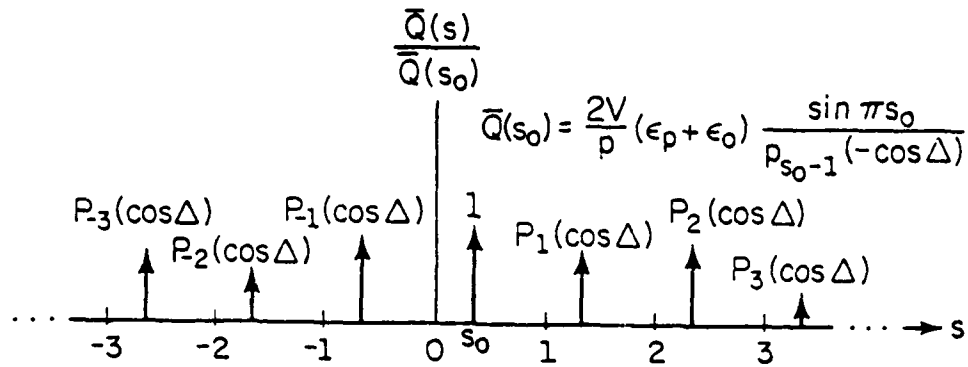
Fig. 14. Fourier transform of charge distribution for a phased array transducer.
