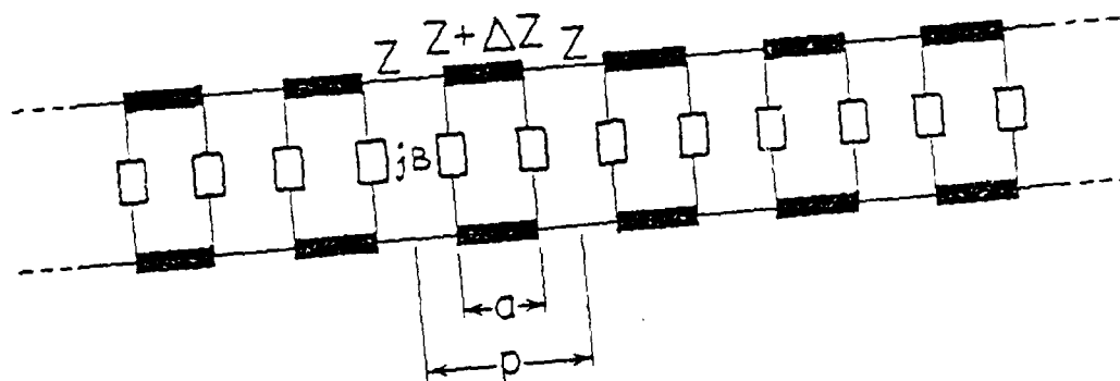
Fig. 4. Surface wave propagation in a periodic array
