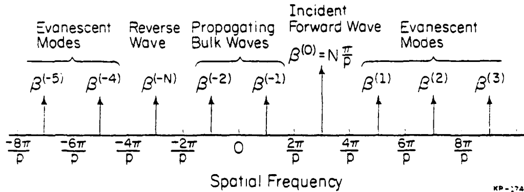
Fig. 6. Spatial harmonics excited by an incident wave in a periodic array at the third harmonic stopband ( N = 3 ).
