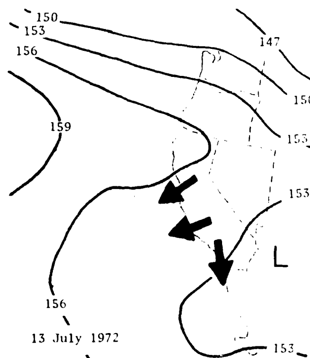
Figure 7. 850-mb Charts for 1200 GMT, 4 July and 13 July 1972.
