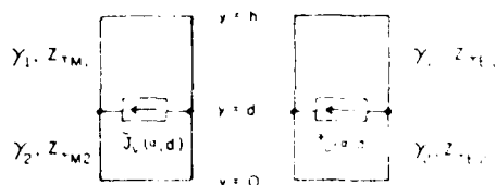
Fig. 3. Equivalent transmission lines for the microstrip line.
