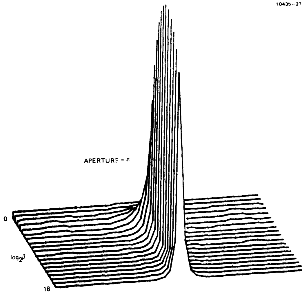
Figure 21. The ME estimates \hat{p}_i^{(o)} , i = 1, \dots, 49 , for aperture size 6 and for 2^0 \leq i \leq 2^{18} .
