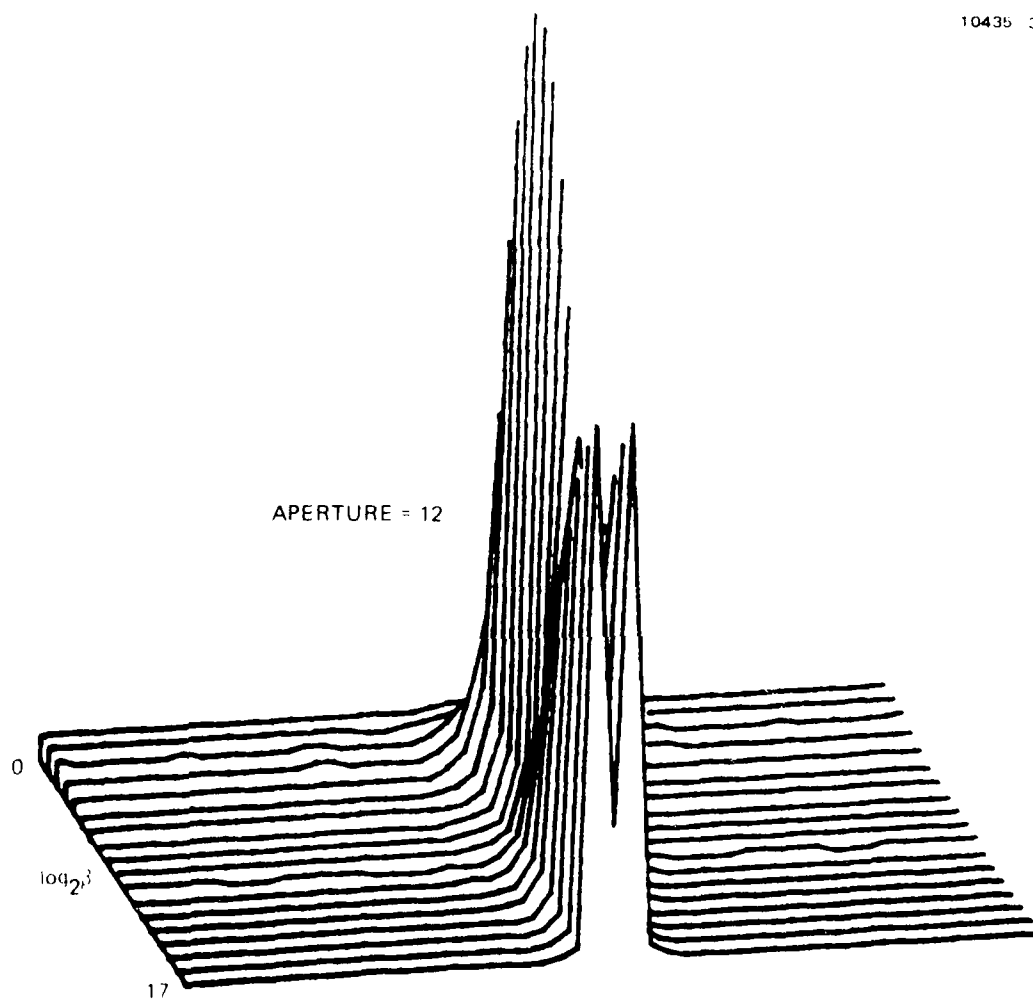
Figure 24. The ME estimates \{p_i^{(0)}\} , 1 \leq i \leq 19 , for aperture size 12 and for 10 \leq i \leq 17 .
