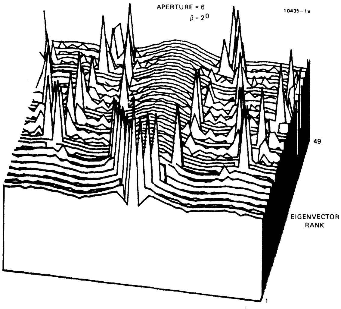
Figure 22(a). Ortho-normal eigenvectors projected on p-space for aperture size 6 and \beta = 2^0 . Positive peaks.
