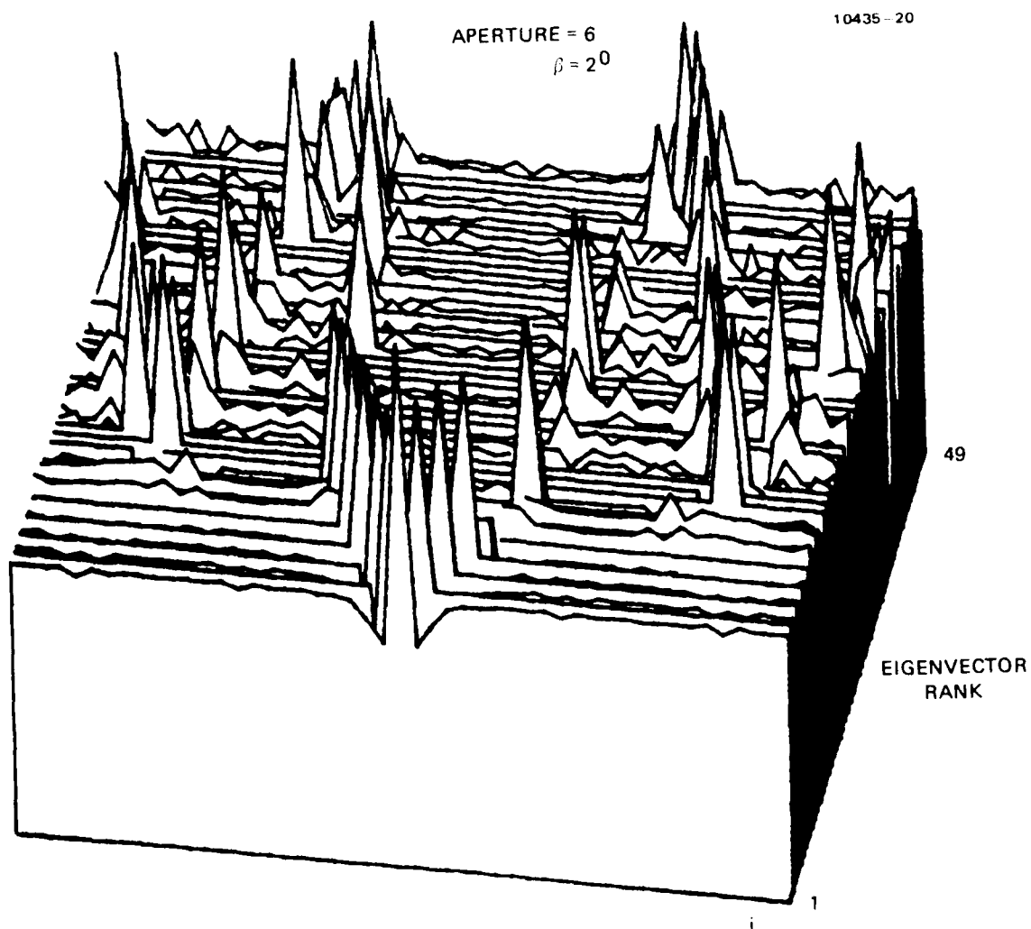
Figure 22(d). The ME estimates \{p_i^{(o)}\} plus 1.05 \{v_i\} for aperture 6, \beta = 2^\circ .
