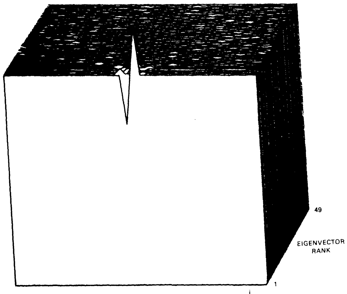
Figure 30(c). Eigenvectors rescaled and projected to p space as \sqrt{2}\{\alpha_i\} for aperture 24, \beta = 2^6 .
