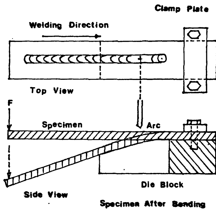
Figure 2: Subsize Varesstraint test equipment (schematic)
