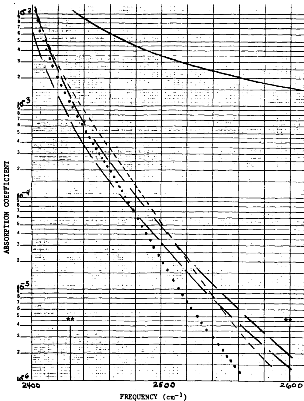
FIGURE 1 - Absorption Coefficient vs Frequency ( \text{cm}^{-1} ), High frequency wing, \nu_3 Band of \text{CO}_2 ; ———, Brackets Experimental Data of Refs. 7,18; ———, Lorentzian Profile; - - - - -, Birnbaum's Theory, \Delta_2 = 27 \text{ cm}^{-1} ; ·····, Birnbaum's Theory, \Delta_2 = 23 \text{ cm}^{-1} ; **, location of other \text{CO}_2 bands.
