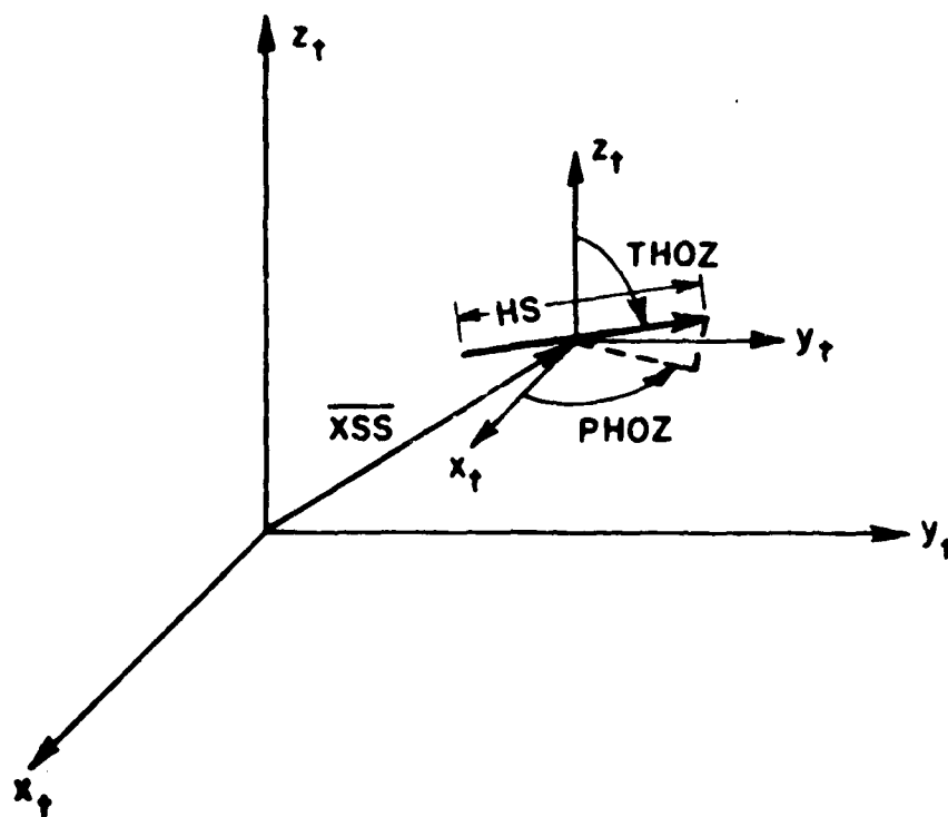
Figure 5a. Definition of source geometry for dipole antennas.
