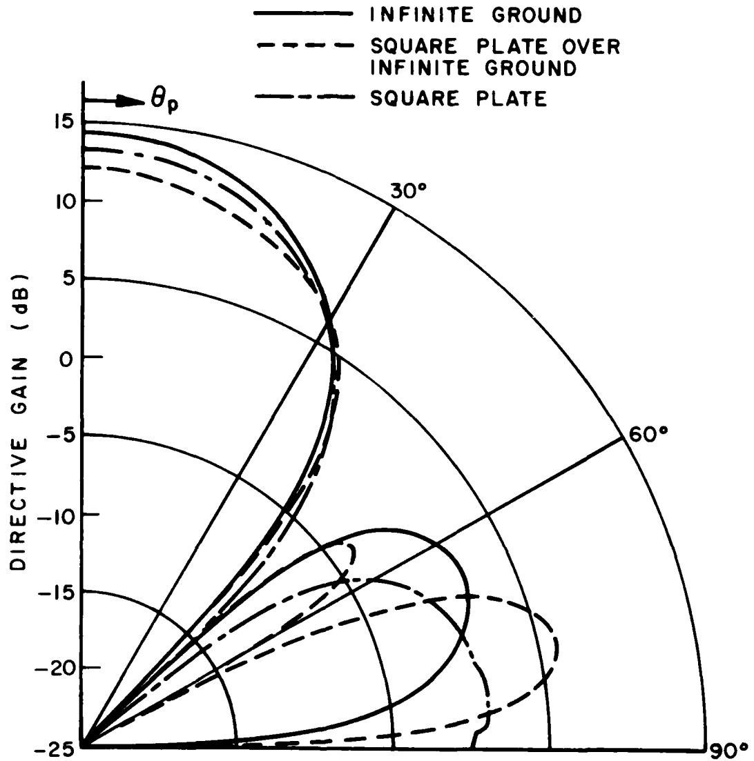
Figure 31b. Comparison of the directive gain of four dipoles over an infinite ground with four dipoles over a square plate over an infinite ground and four dipoles over a square plate alone ( \phi=90^\circ , horizontal polarization).
