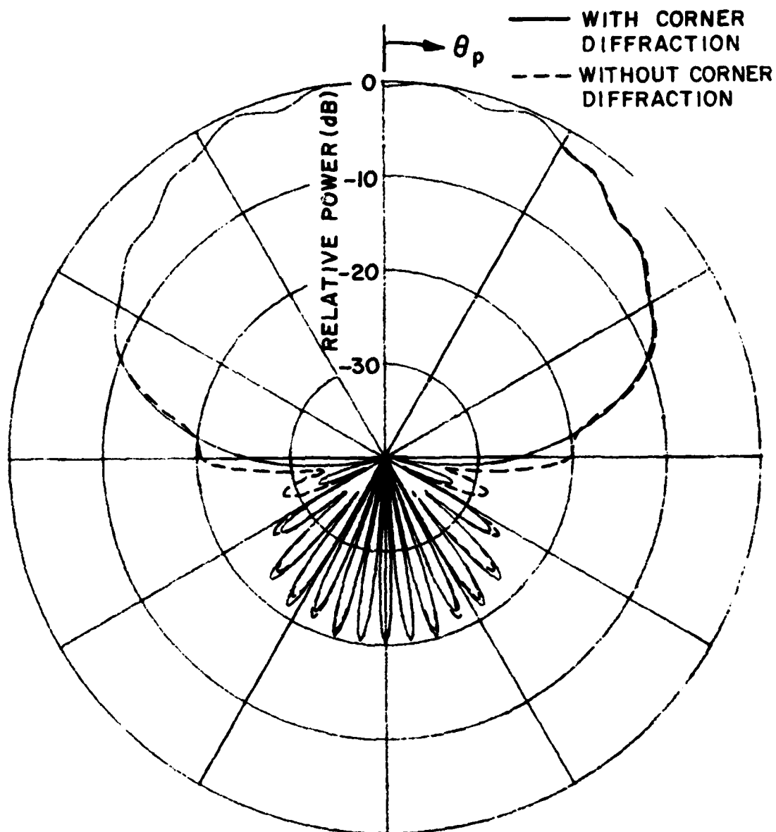
Figure 15b. Comparison of E_{\theta} pattern with and without corner diffracted fields for a half-wave slot antenna mounted on a square plate.
