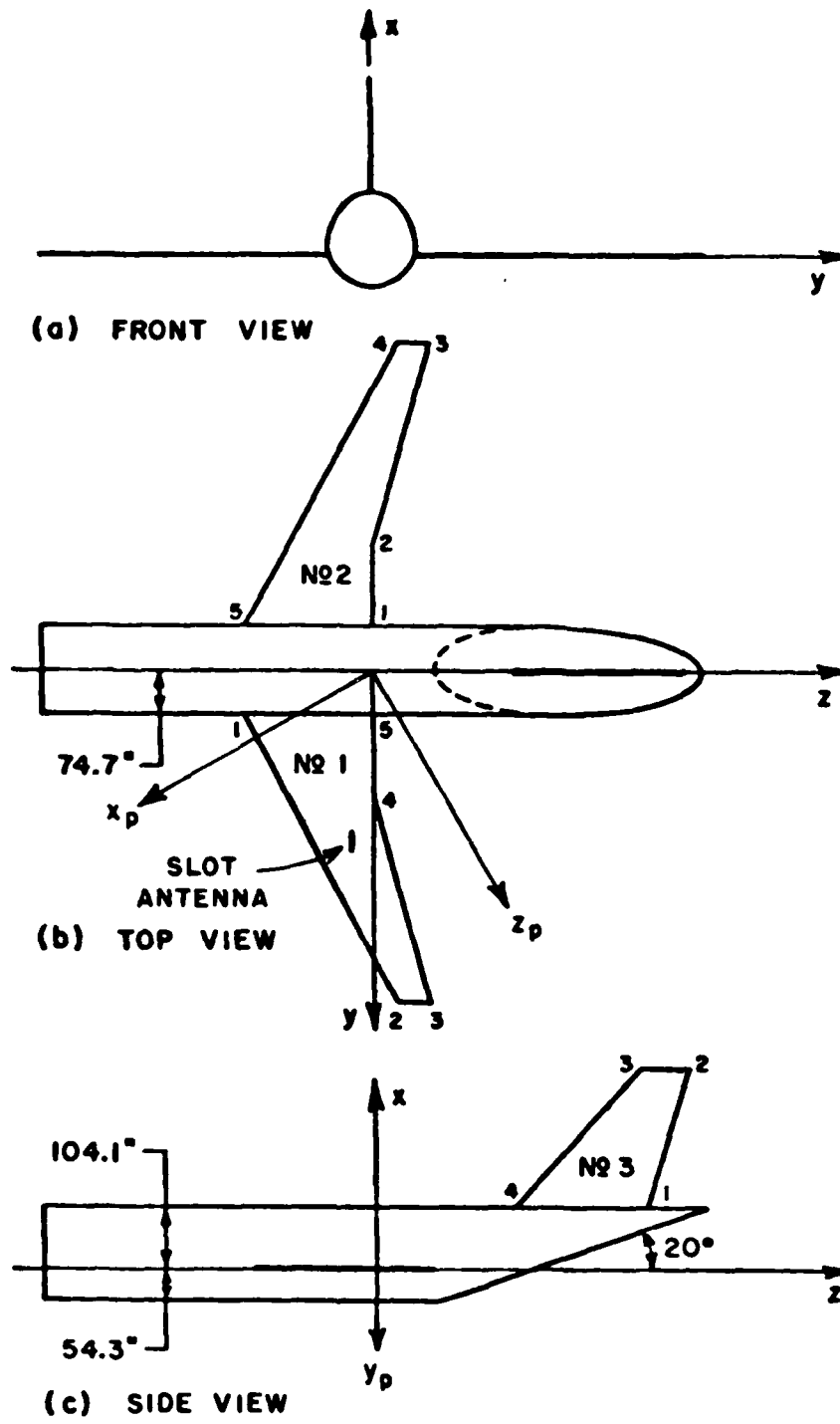
Figure 27. Illustration of geometry of Boeing 737 aircraft model used in finite elliptic cylinder model.
