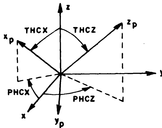
Figure 1a. Definition of pattern coordinate system.
