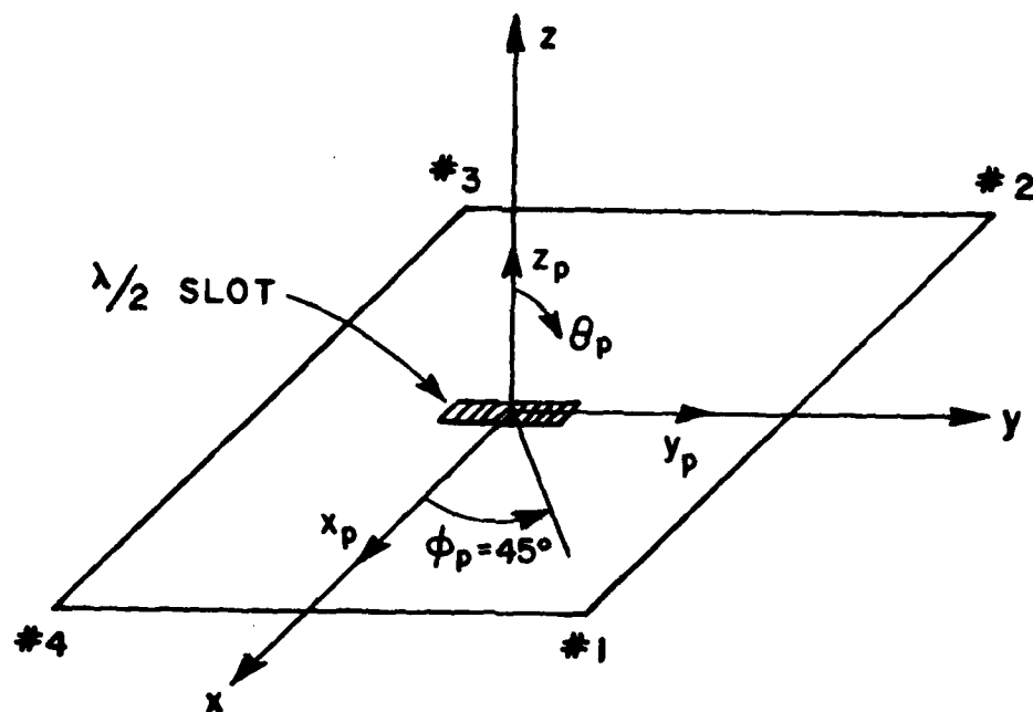
Figure 14. A \lambda/2 slot mounted on top of a square ground plane.
