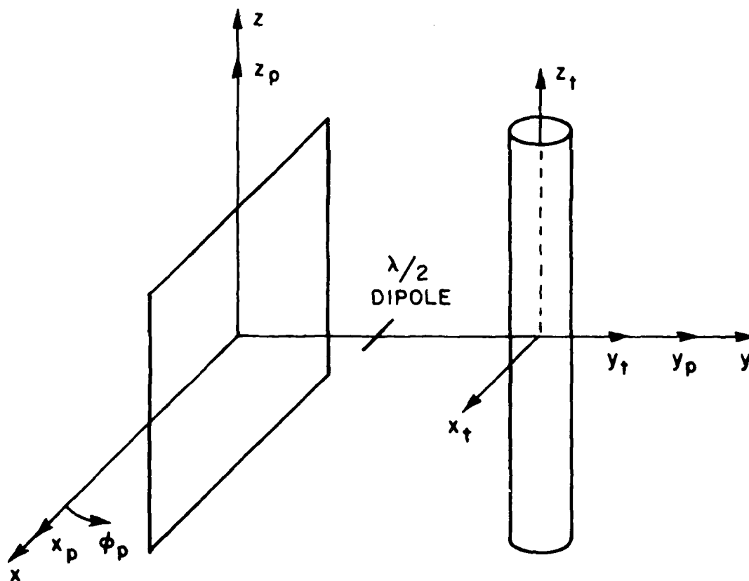
Figure 24. A \lambda/2 dipole in the presence of a square plate.
