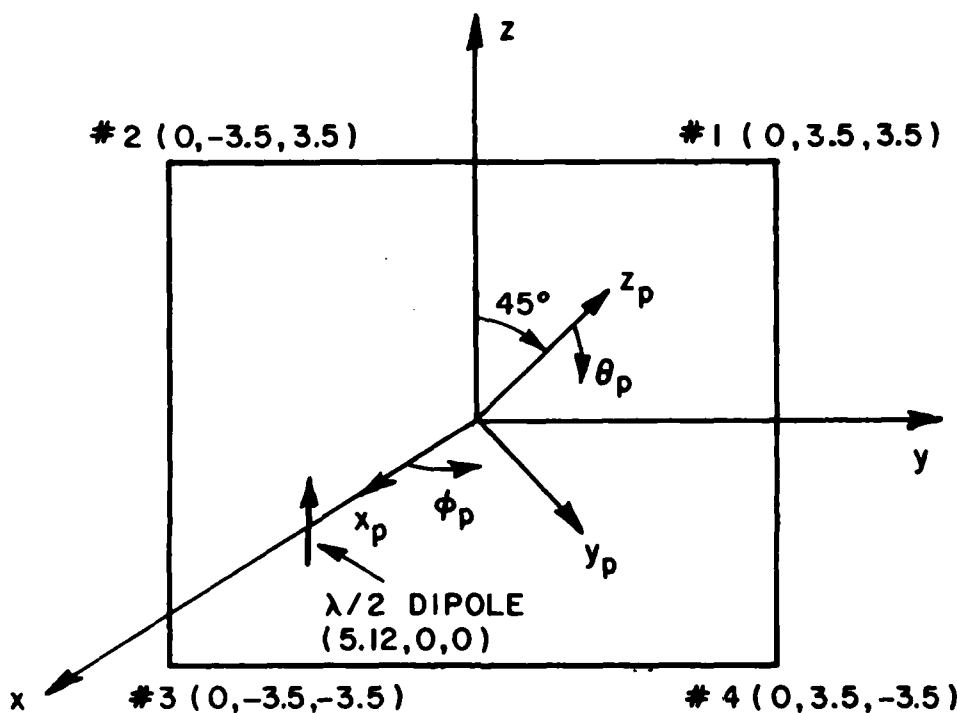
Figure 10b. Dipole in presence of a square ground plane with a pattern cut corresponding to Example 1c.
