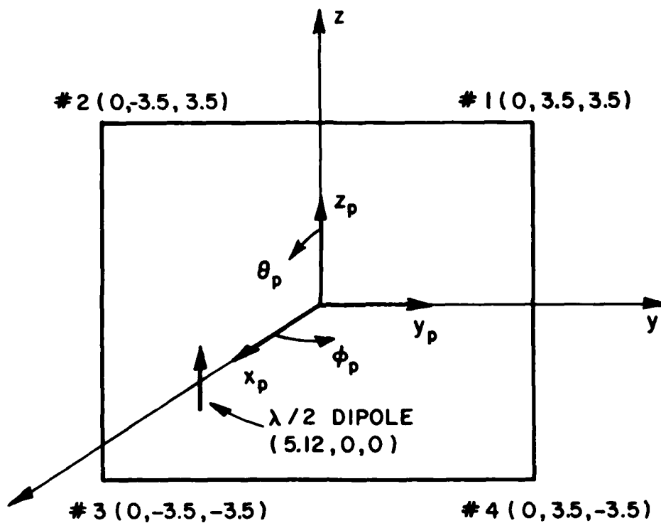
Figure 10a. Dipole in presence of a square ground plane.
