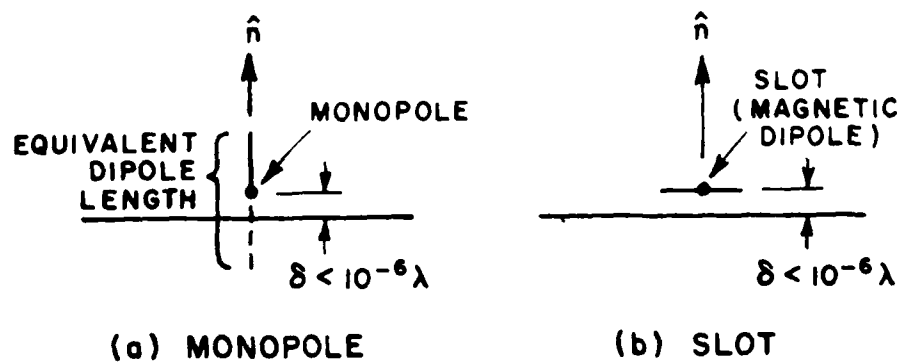
Figure 9. Illustration of geometry for plate-mounted antennas.
