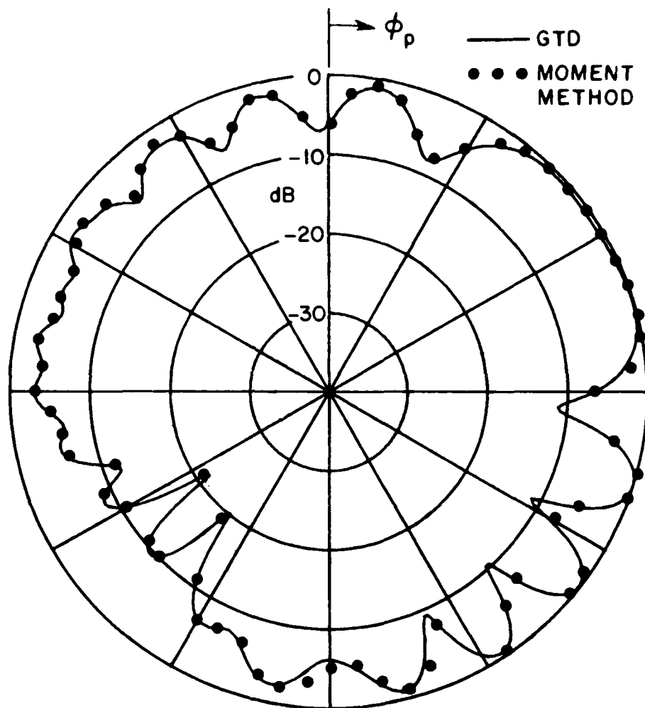
Figure 23. Comparison of GTD and moment method results for E_{\phi_p} pattern.
