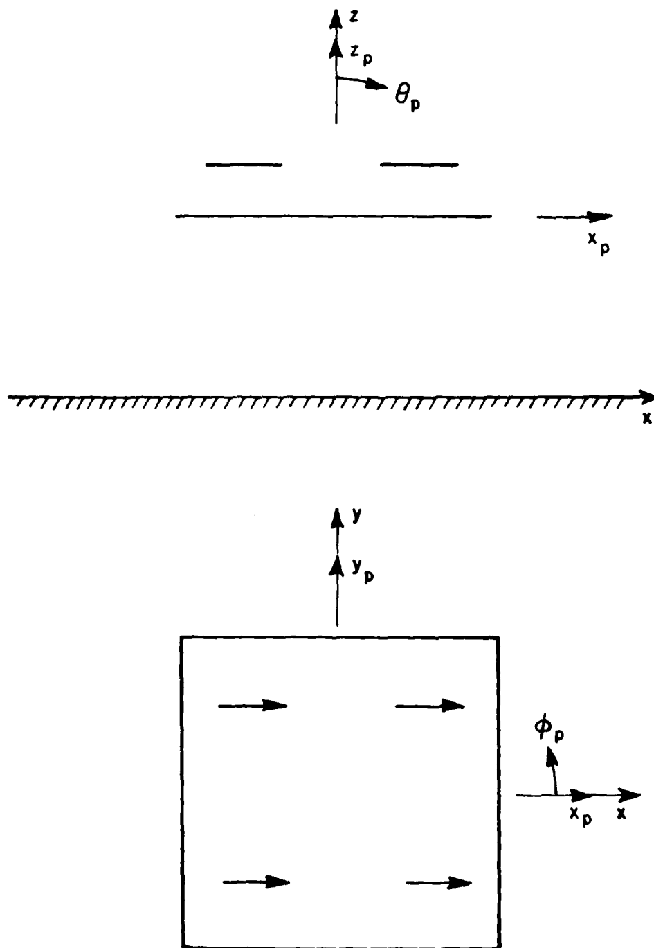
Figure 29. Geometry for the problems of dipoles over a square plate and infinite ground plane showing the side and top view.
