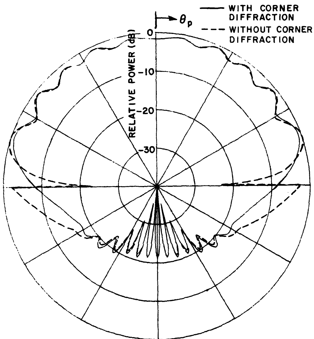
Figure 15a. Comparison of E_{\theta p} pattern with and without corner diffracted fields for a half-wave slot antenna mounted on a square plate.
