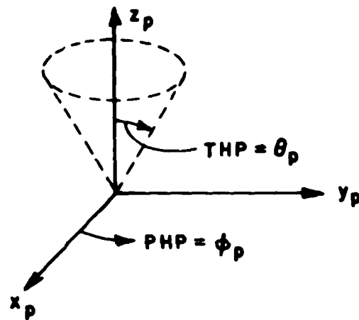
Figure 1b. Conic pattern cut, LCNPAT=.TRUE., TPPD=THP.
