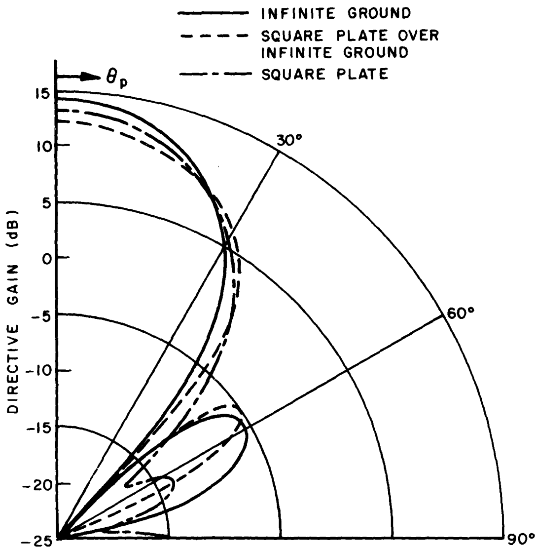
Figure 31a. Comparison of the directive gain of four dipoles over an infinite ground with four dipoles over a square plate over an infinite ground and four dipoles over a square plate alone ( \phi=0^\circ , vertical polarization).
