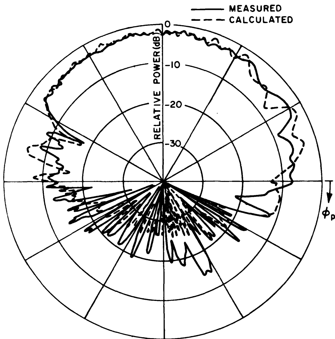
Figure 28. Comparison of measured and calculated E_{\theta_p} results.
