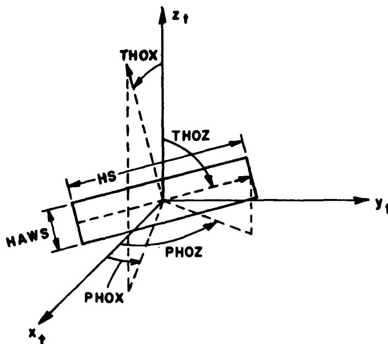
Figure 5b. Definition of source geometry for aperture antennas.
