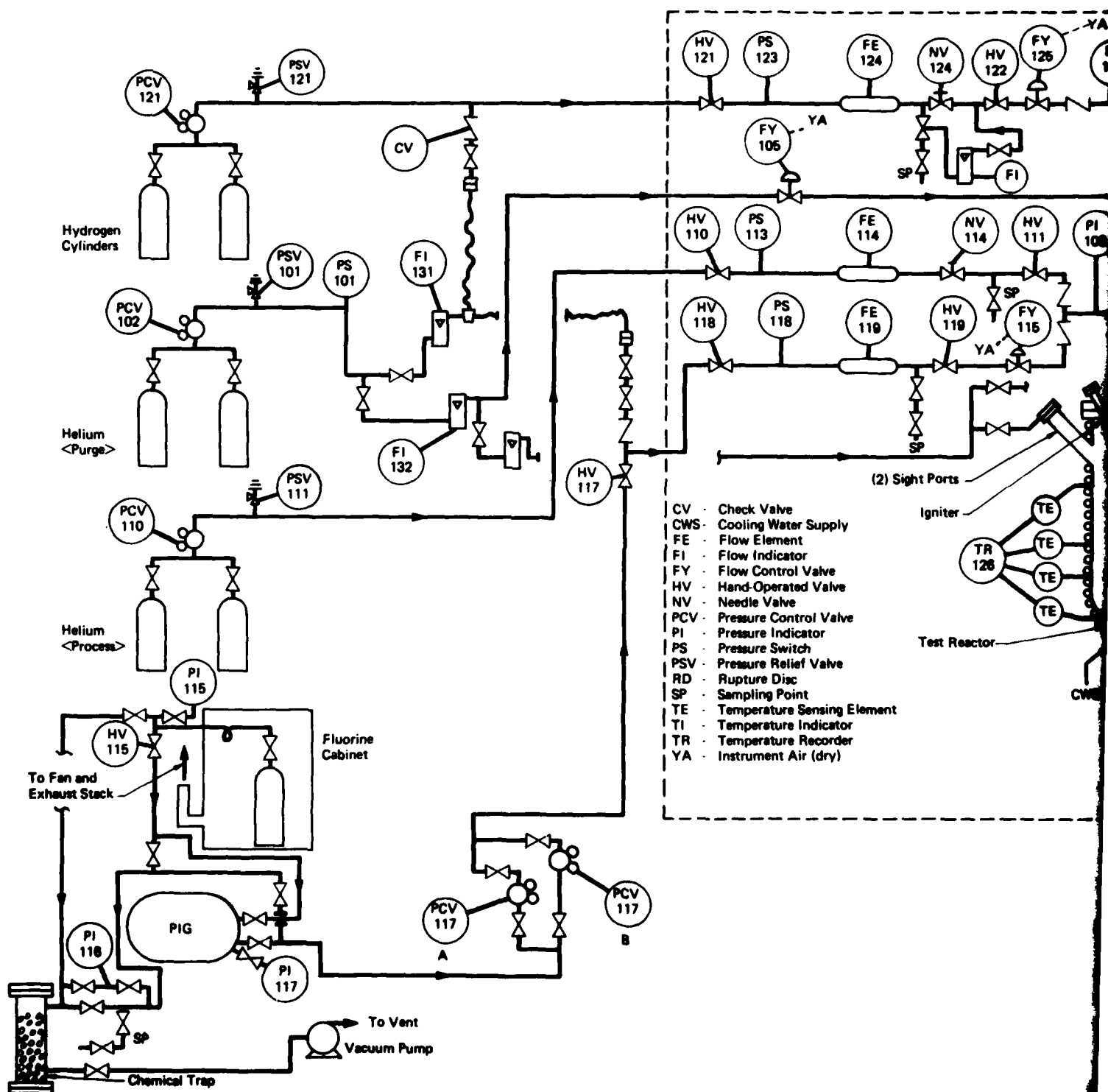
Figure 1. MATERIAL TEST FACILITY FLOW DIAGRAM.
