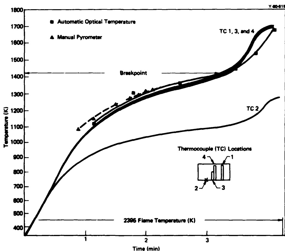
Figure 27. TEMPERATURE-VERSUS-TIME CURVE FOR NICKEL 270 EXPOSED TO HYDROGEN FLUORINE FLAME. (Run HF-140.)
