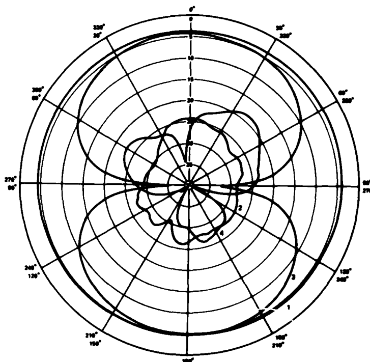
Figure A-19. Loop antenna 735-1 radiation pattern measurements at 735 MHz.
