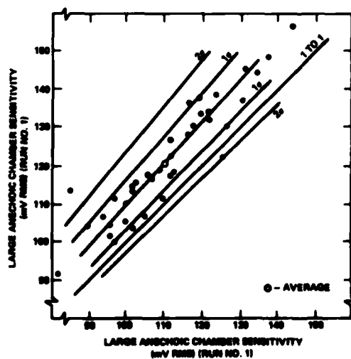
Figure 14. Correlation plot for two runs in large anechoic chamber.
