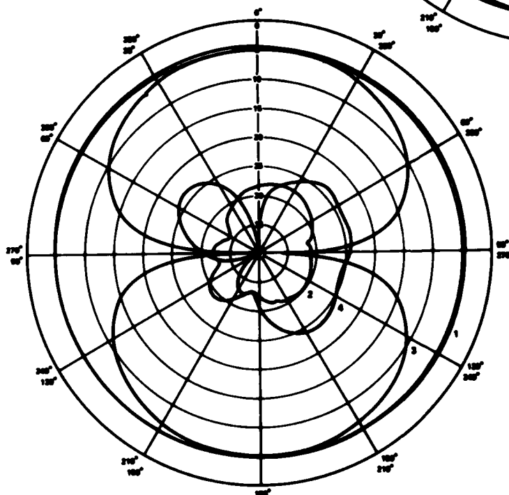
Figure A-34. Loop antenna 700-2 radiation pattern measurements at 700 MHz.
