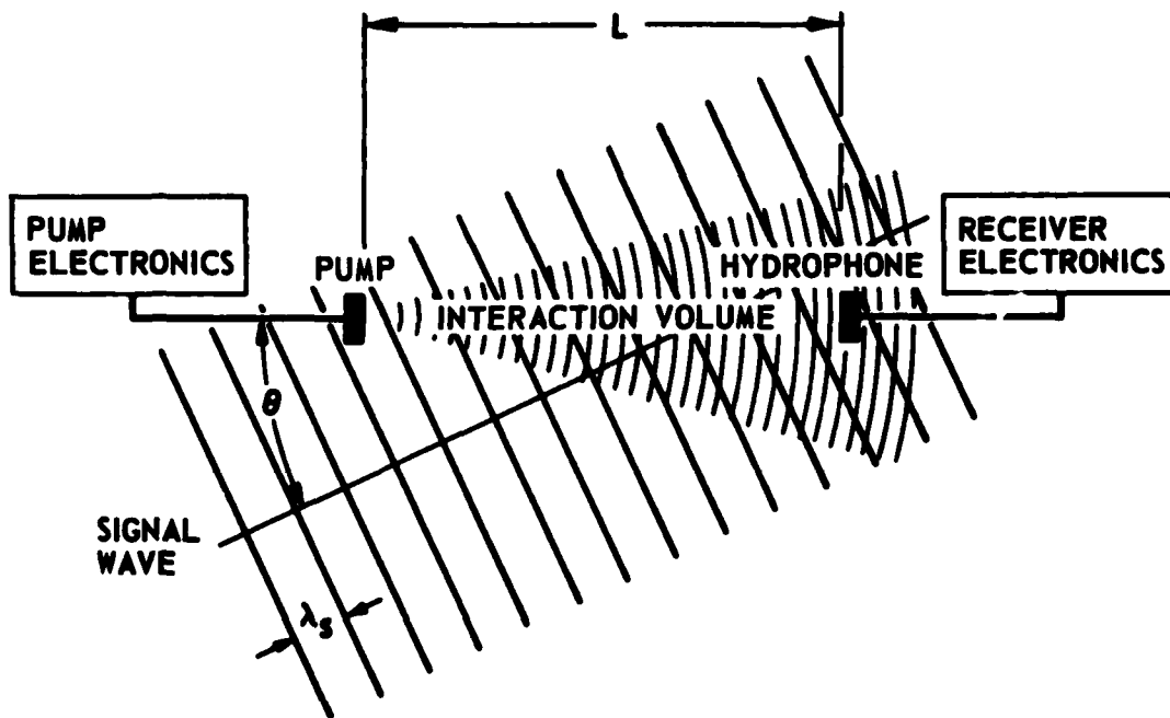
FIGURE 1 PARRY FUNCTIONAL DIAGRAM
