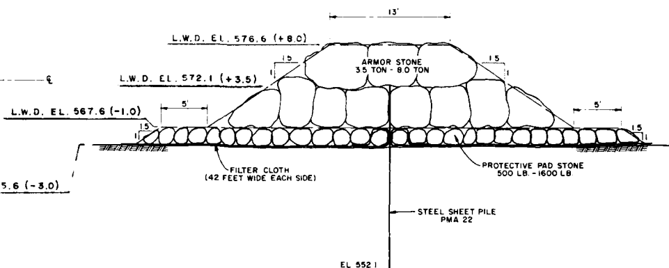
TYPICAL HEAD SECTION
