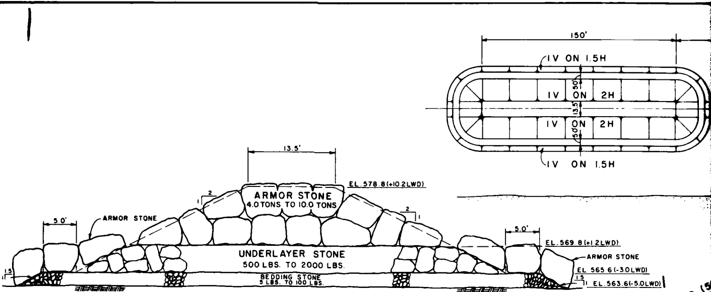
TYPICAL SECTION SCALE OF FEET 0 6 12
