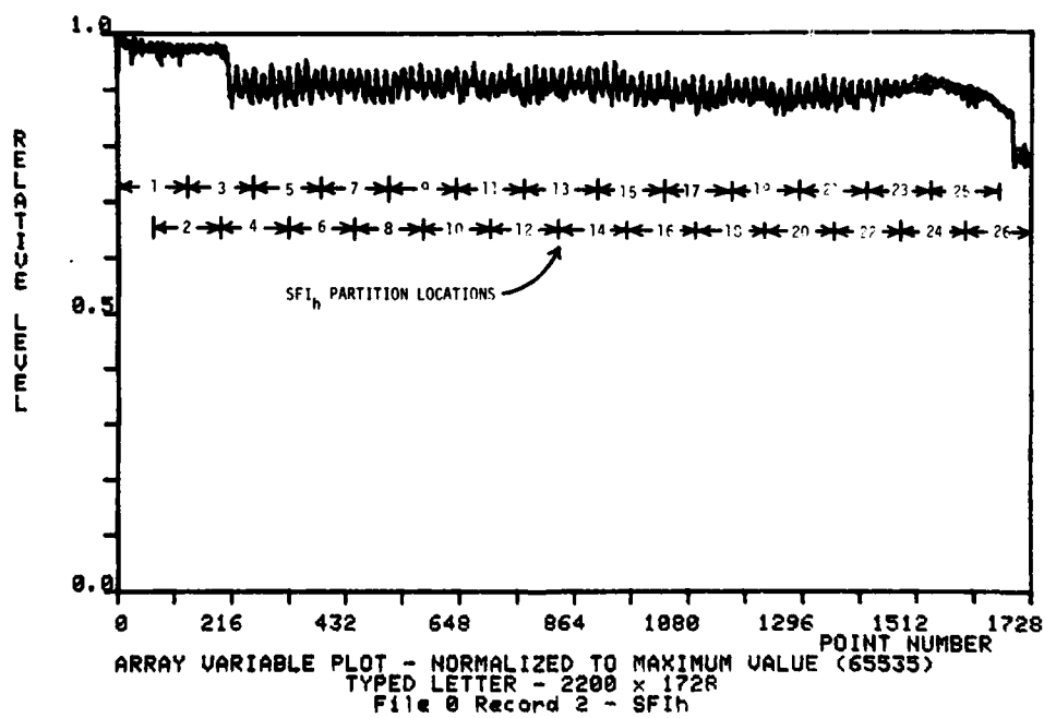
Figure C23. Typewritten text without justification - SFI h partition locations.
