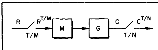
Figure 6. Fast-Input/Slow-Output Sampling with Common Sampling Period T
