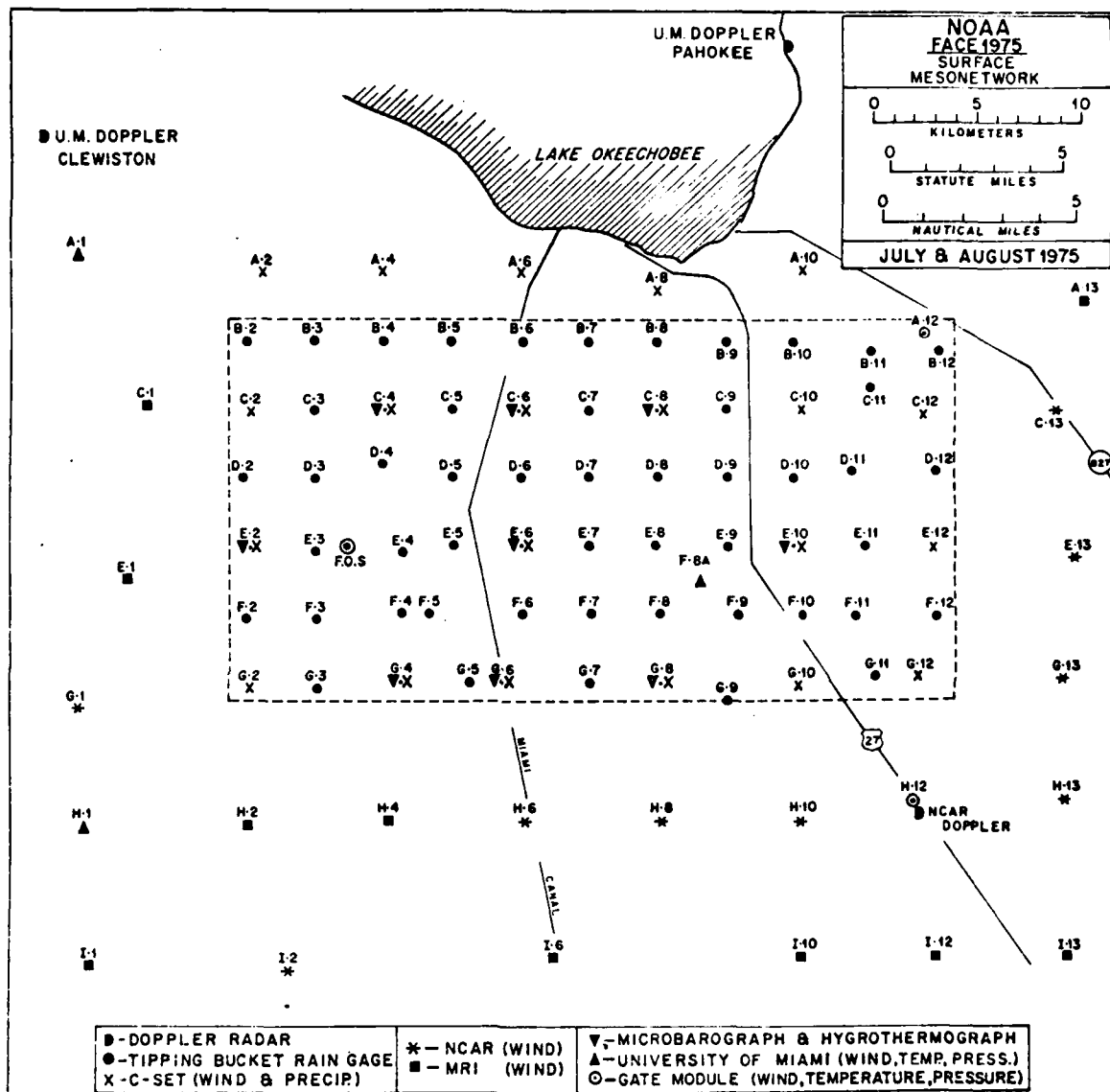
Figure 2. FACE 1975 mesonetwork. The dashed line encloses the rain gage cluster. Locations of the Doppler radar sites and Field Observing Site (FOS) are also shown.
