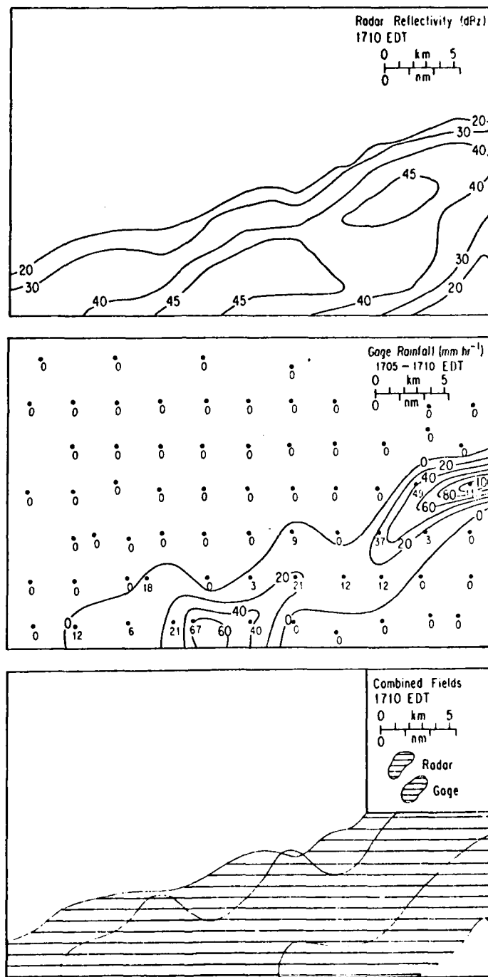
Figure 22. Upper panel: radar echo pattern from Miami WSR-57 at 1710 EDT. Middle panel: rain gage data and isohyet analysis for 1705 to 1710 EDT. Lower panel: combined data superimposed.
