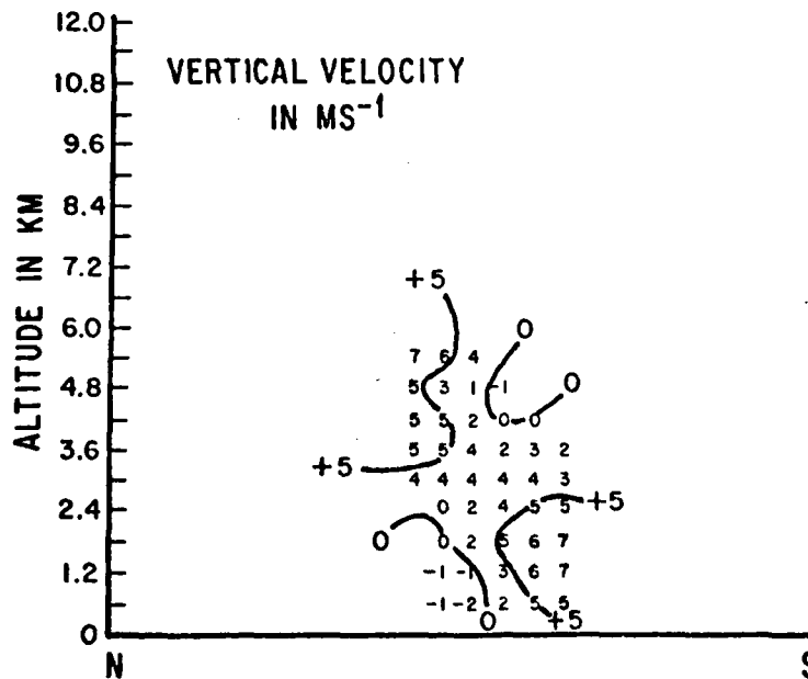
Figure 31. Vertical cross section of reflectivity and vertical velocity at 1431 EDT on 25 August 1975. Sections are approximately north-south through cell A as shown in Figure 28. Upper panel: reflectivity in 5-dBz increments, beginning at 15 dBz. Lower panel: vertical velocity in \text{ms}^{-1} . Positive indicates upward flow. Data plotted at 600 m intervals.
