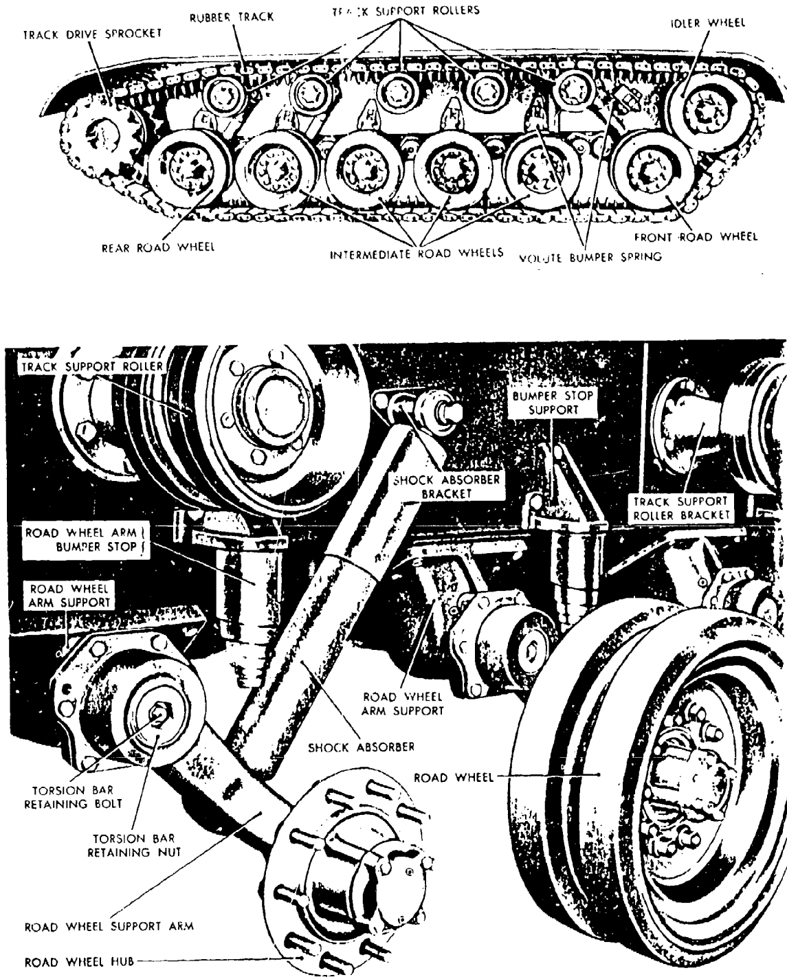
Figure 3. Suspension system components.
