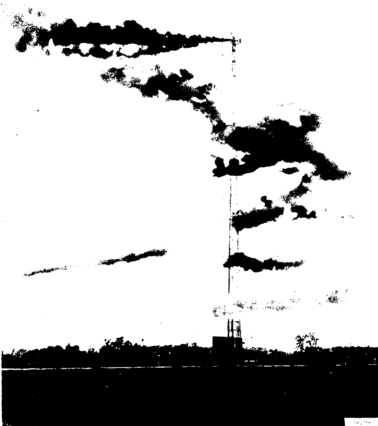
FIGURE 1. SMOKE STREAMS SHOWING 180° WIND DIRECTION CHANGE WITHIN 140 FEET OF GROUND. FLAT TERRAIN
