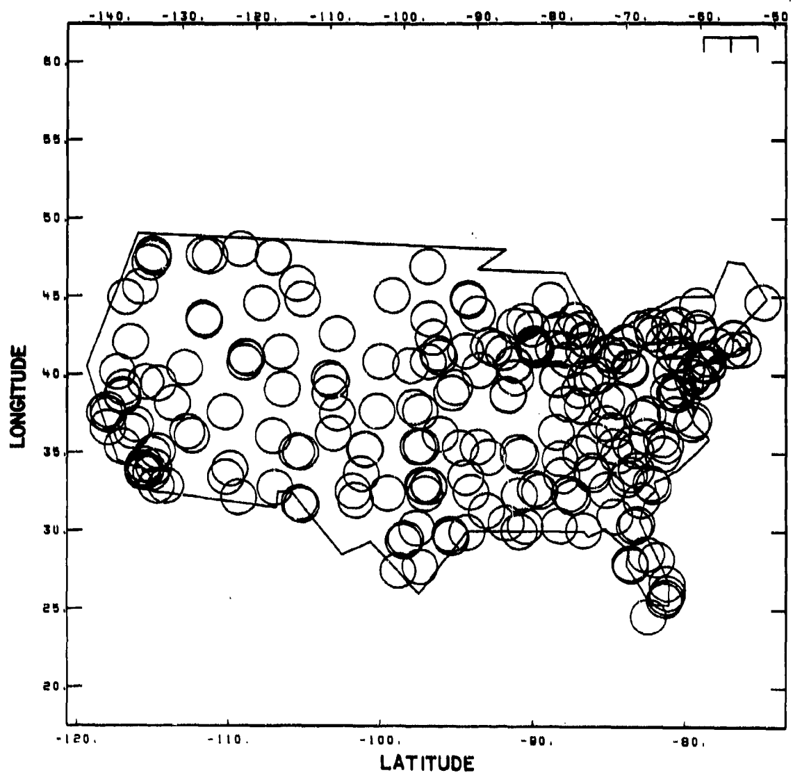
Fig. B.2. Radar coverage at 4000 feet AGL for 243 sensor network.
