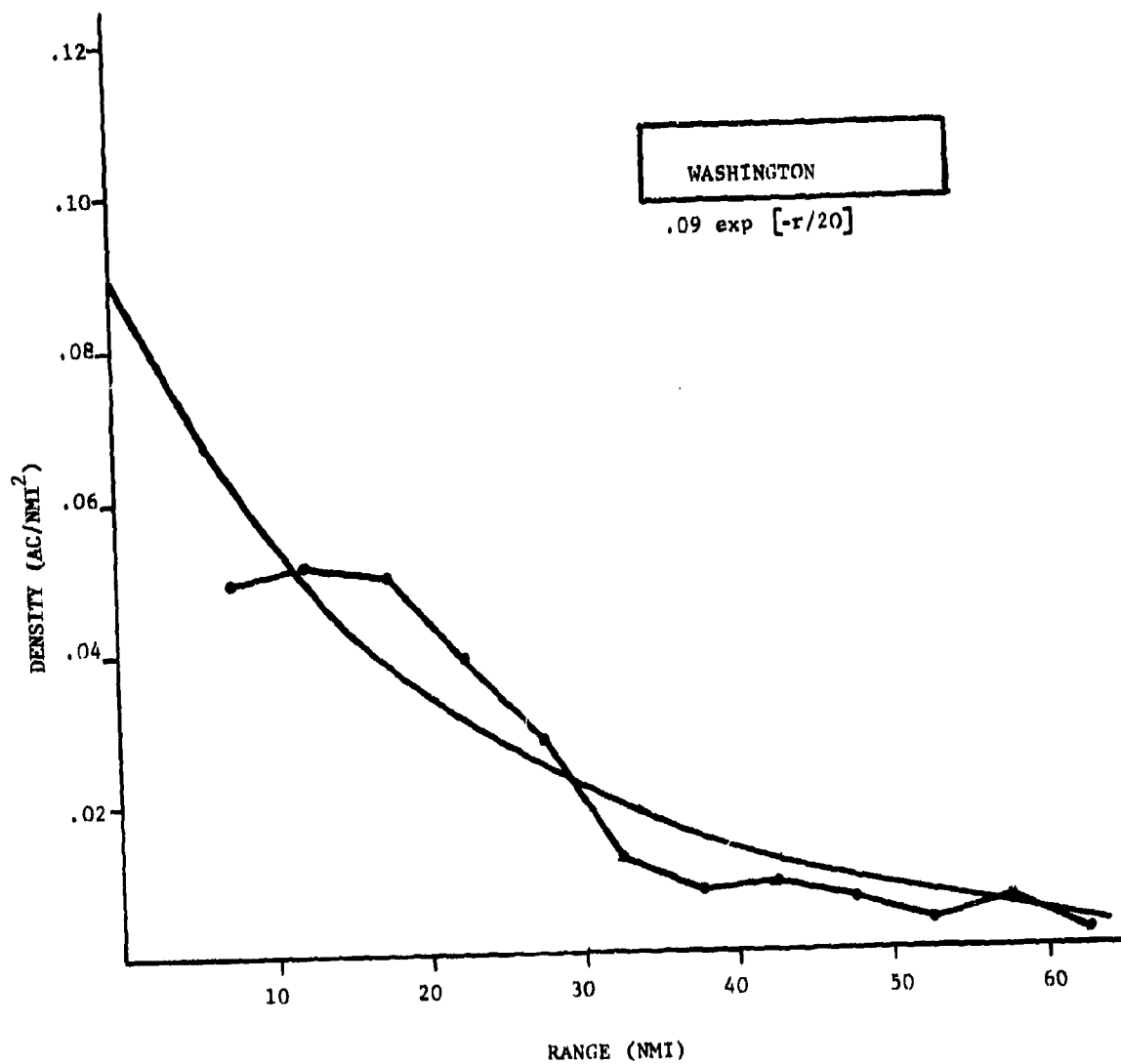
Fig. C.6. Exponential fit to TMF traffic data at Washington.
