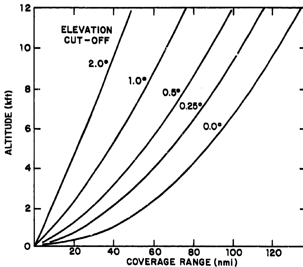
Fig. B.1. Radar coverage altitude versus range from sensor. An elevation cut-off angle of 0.25^\circ was selected for purposes of coverage analysis.
