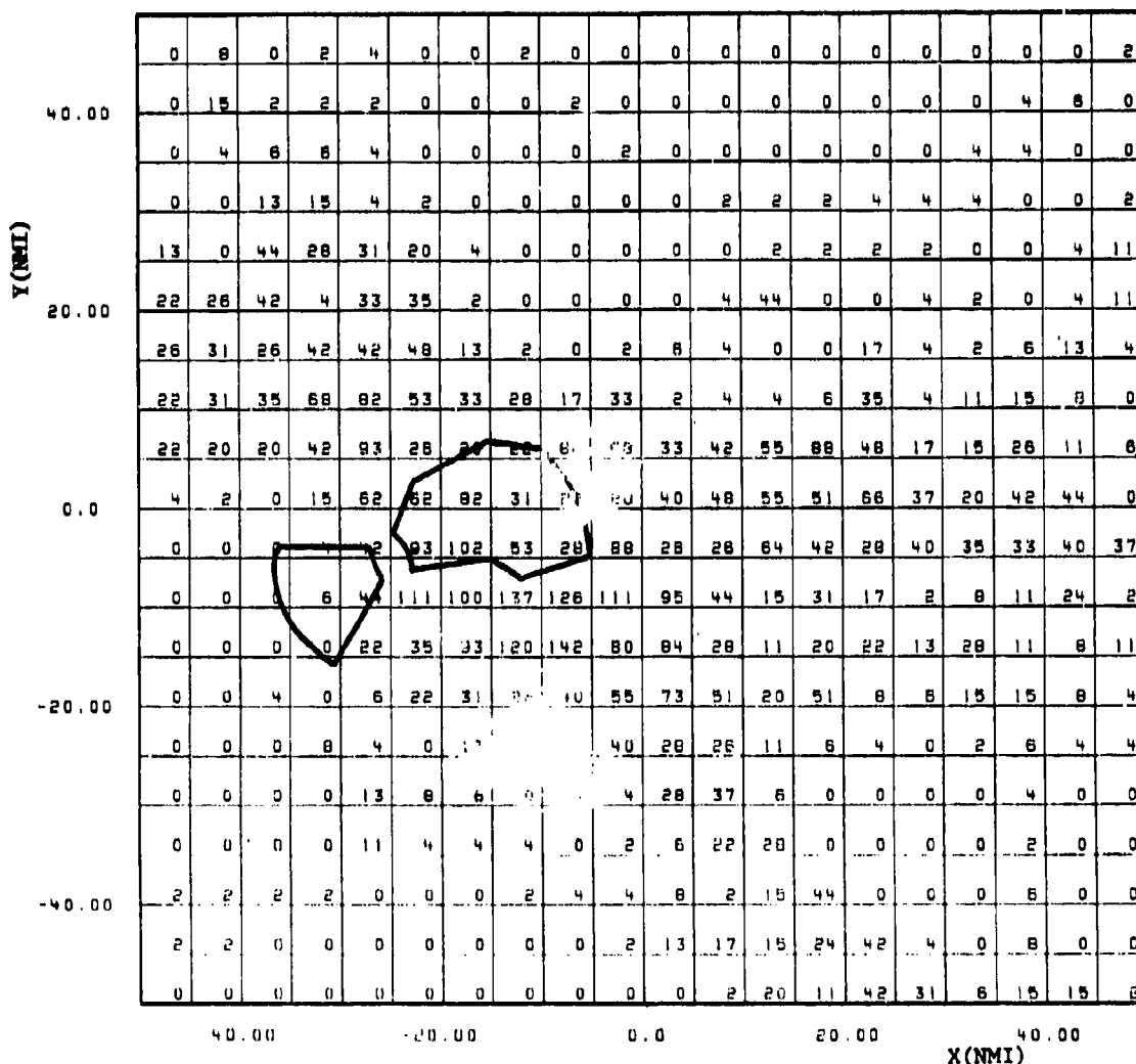
Fig. C.4. Aircraft density (aircraft per 1000 nmi 2 ) observed by sensor near Los Angeles (Brea). The outline approximates the Los Angeles TCA boundary at 3000 feet.
