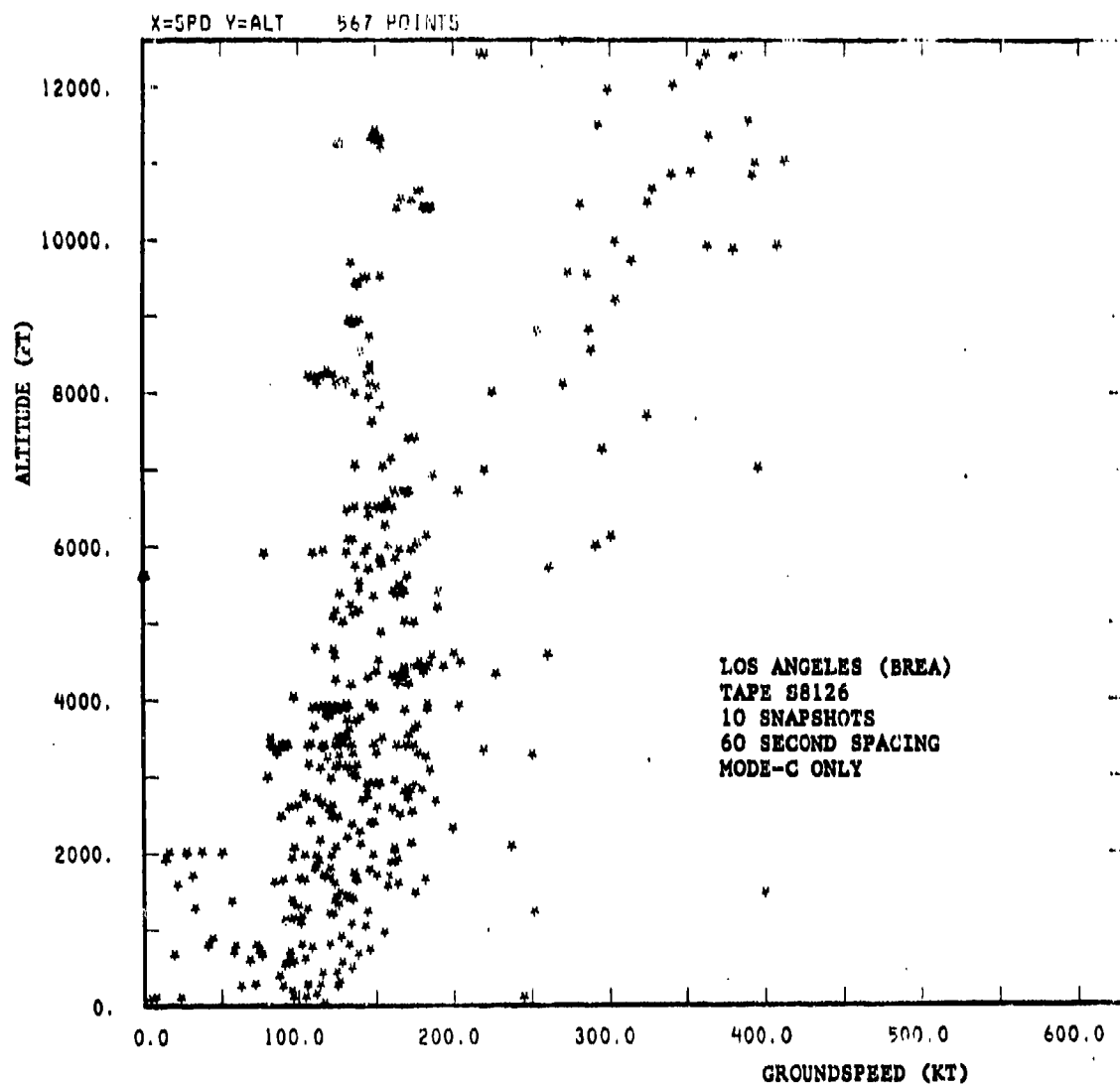
Fig. C.1. Altitude versus groundspeed for mode-C reporting aircraft observed by sensor near Los Angeles (Brea). The plot combines data from 10 snapshots spaced at 60 second intervals.
