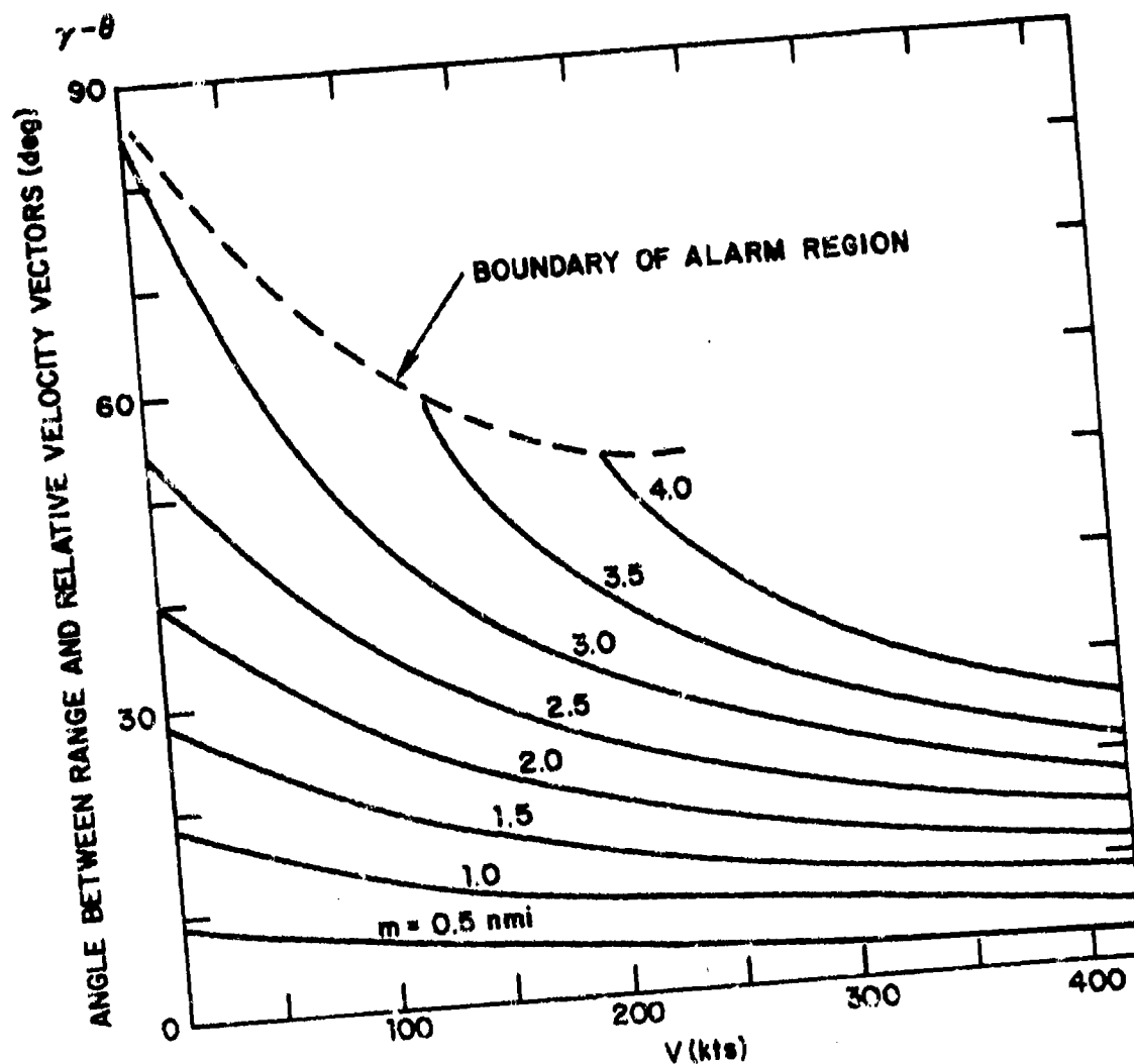
Fig. A.7. Angle between range and relative velocity vectors at time modified tau criterion is violated for \tau = 60 seconds, r_0 = 3.0 \text{ nmi} .
