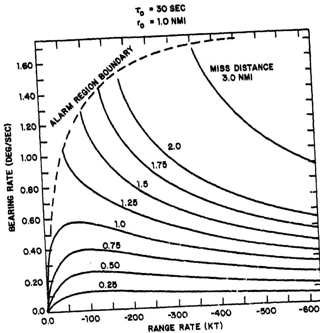
Fig. A.3. Bearing rate at time of detection versus range rate at time of detection.
