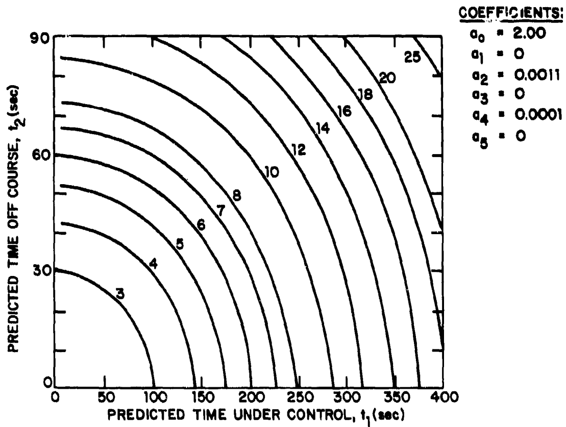
Fig. D.3. Contours of control cost.
