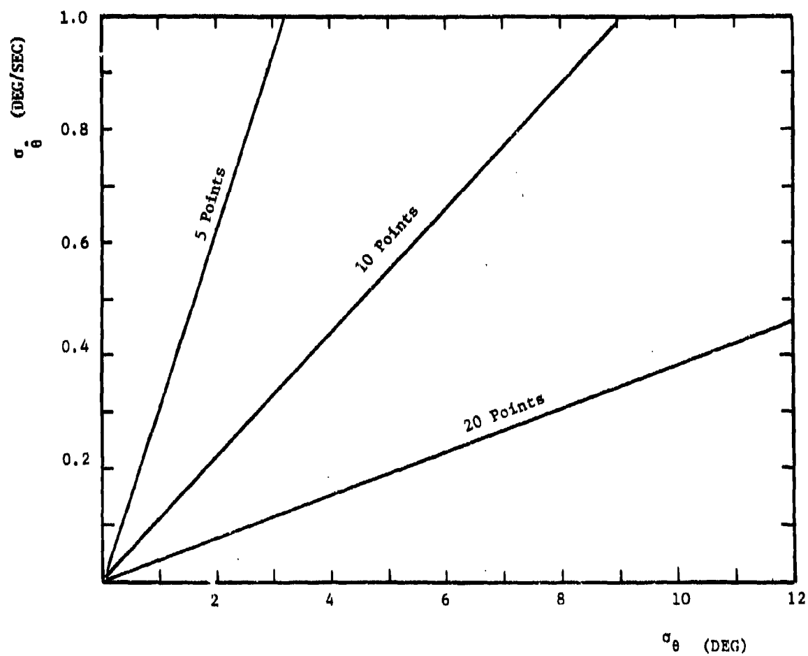
Fig. A.6. Bearing rate estimation error (1 sec. update rate).
