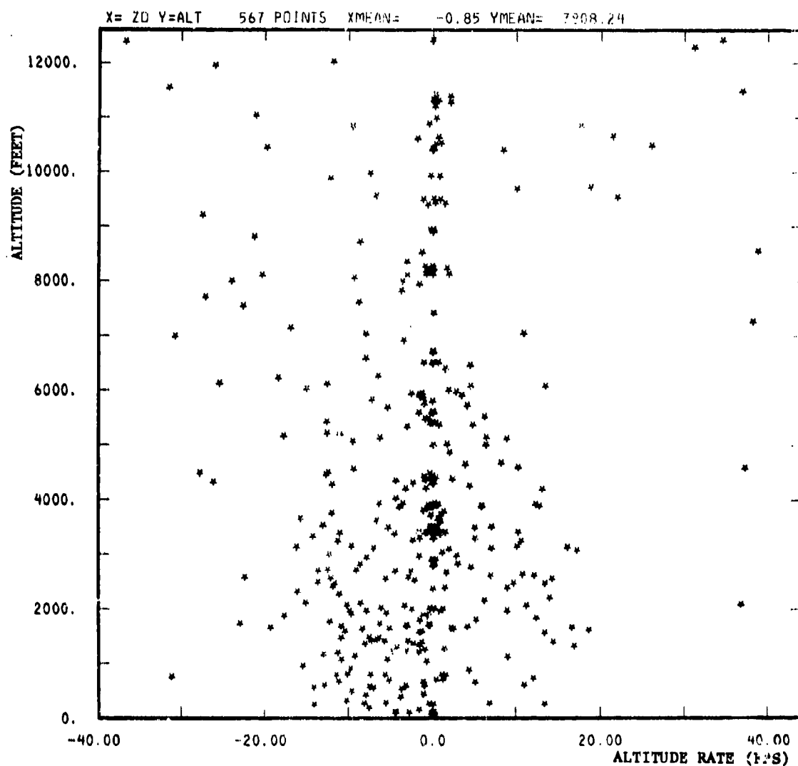
Fig. C.3. Altitude versus altitude rate for Mode-C reporting aircraft observed by sensor near Los Angeles (Brea). The plot combines data from 10 snapshots spaced at 60 second intervals.
