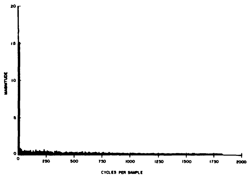
Figure 4-14. Spectrum for daily average temperature, Madison, WI (1953-1962).
