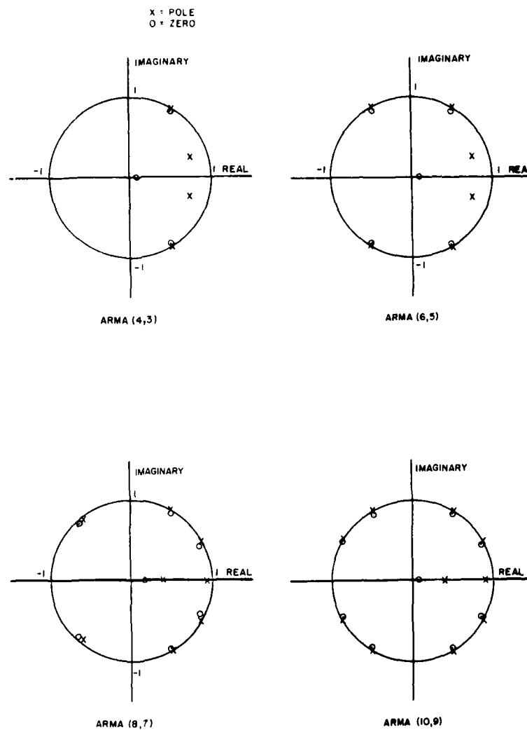
Figure 4-5. Pole-zero plots for successive ARMA models for dry-bulb temperature, Charleston, SC.
