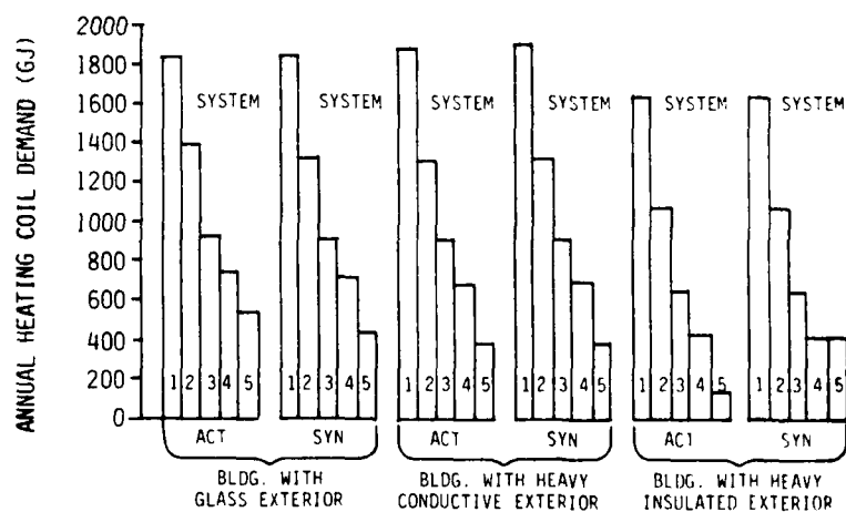
Figure 5-17. Annual heating coil demand, Madison, WI.
