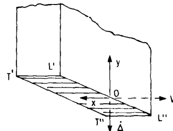
(a) View of blade rub surface L'L''T'T' moving with velocity V and rate of incursion \Delta relative to seal material.
