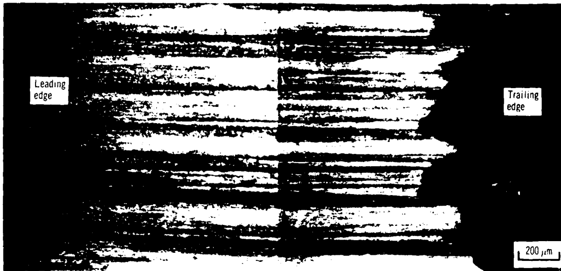
Figure 12. - Rounded Ti-6Al-4V blade tip after rub interaction against 21-percent-dense, sintered Hastelloy-X fibermetal. Blade tip velocity, 114 m/sec; incursion rate, 25 \times 10^{-6} m/sec.
