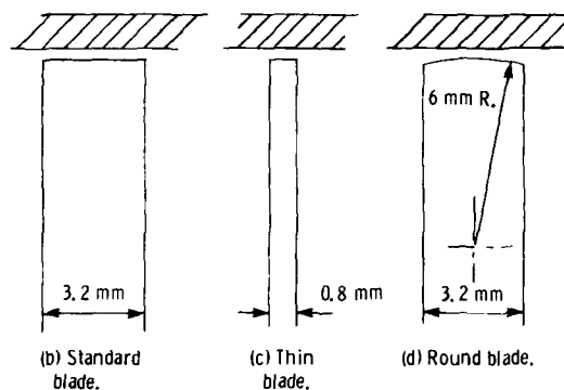
Figure 1. - Test apparatus and sections through blade tips.
