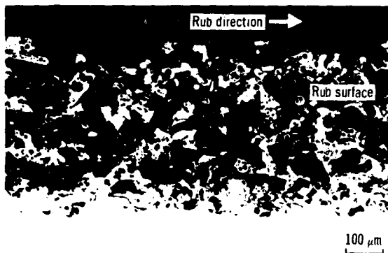
Figure 13. - Metallographic section through rub groove on plasma-sprayed Ni-25-percent graphite after interaction with thin Ti-6Al-4V blade tips. Blade tip velocity, 114 m/sec; incursion rate, 25 \times 10^{-6} m/sec.
