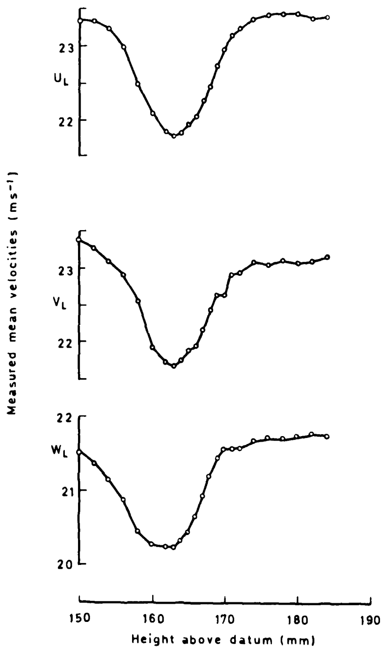
Fig 4 Vertical traverse through wake (221 mm in from wing-tip, 3% chords downstream)
