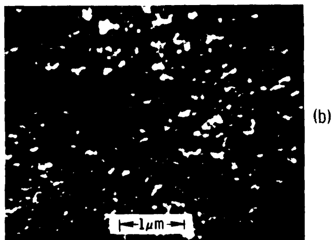
Fig. 2. A comparison of the coverages obtained with high-field pulse-plating and dc plating methods. The light areas are plated Pt; the dark areas are the base GaAs surface. (a) High-field pulse-plating of Pt. (b) DC plating of Pt.
