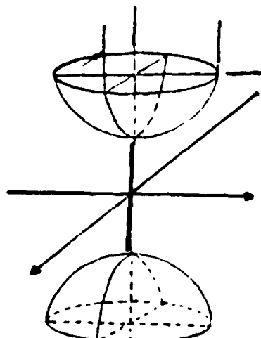
ELLIPTIC HYPERPOLID OF 2 SHEETS
