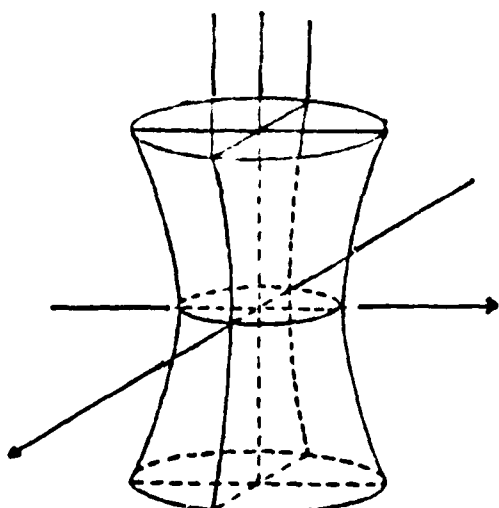
ELLIPTIC HYPERBOLOID OF 1 SHEET
