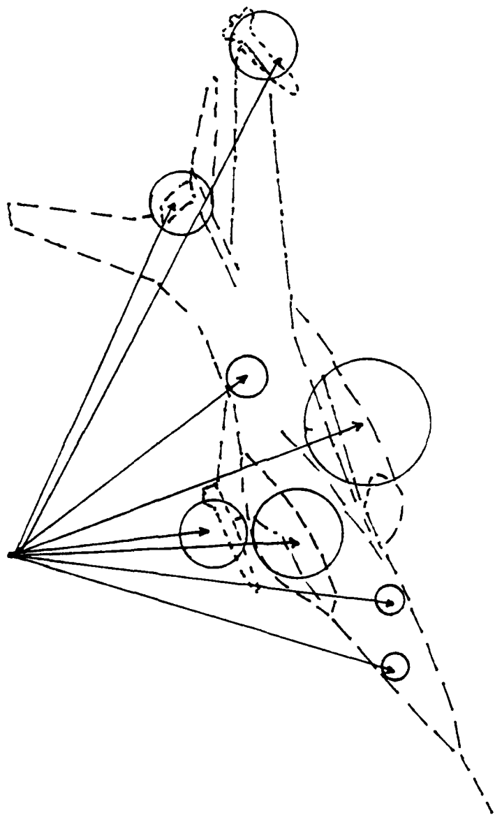
Figure 2-5 Example of ATTACK Single Fragment (Component) Model
