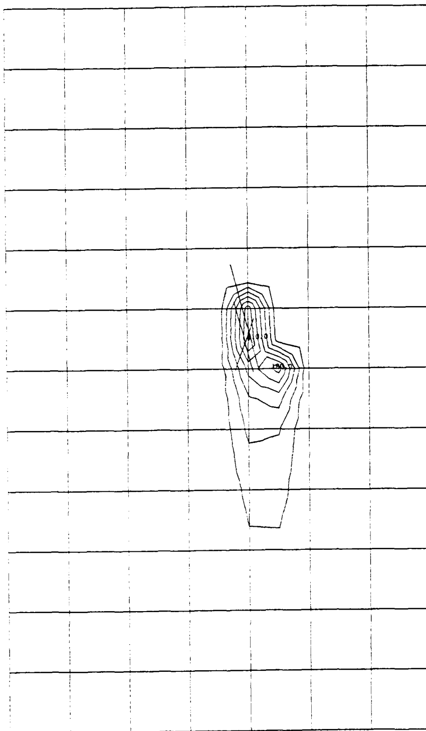
AIRCRAFT PT CONCENTRATION PROFILE (6 AUG 1515-1615) INCREMENTED FROM 30.0
