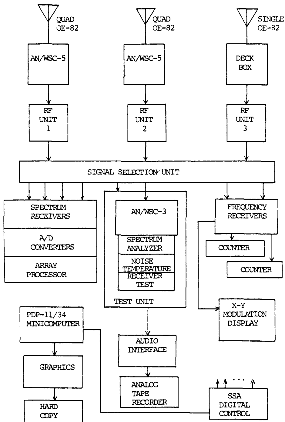
FIGURE 1.1. SSA BLOCK DIAGRAM.
