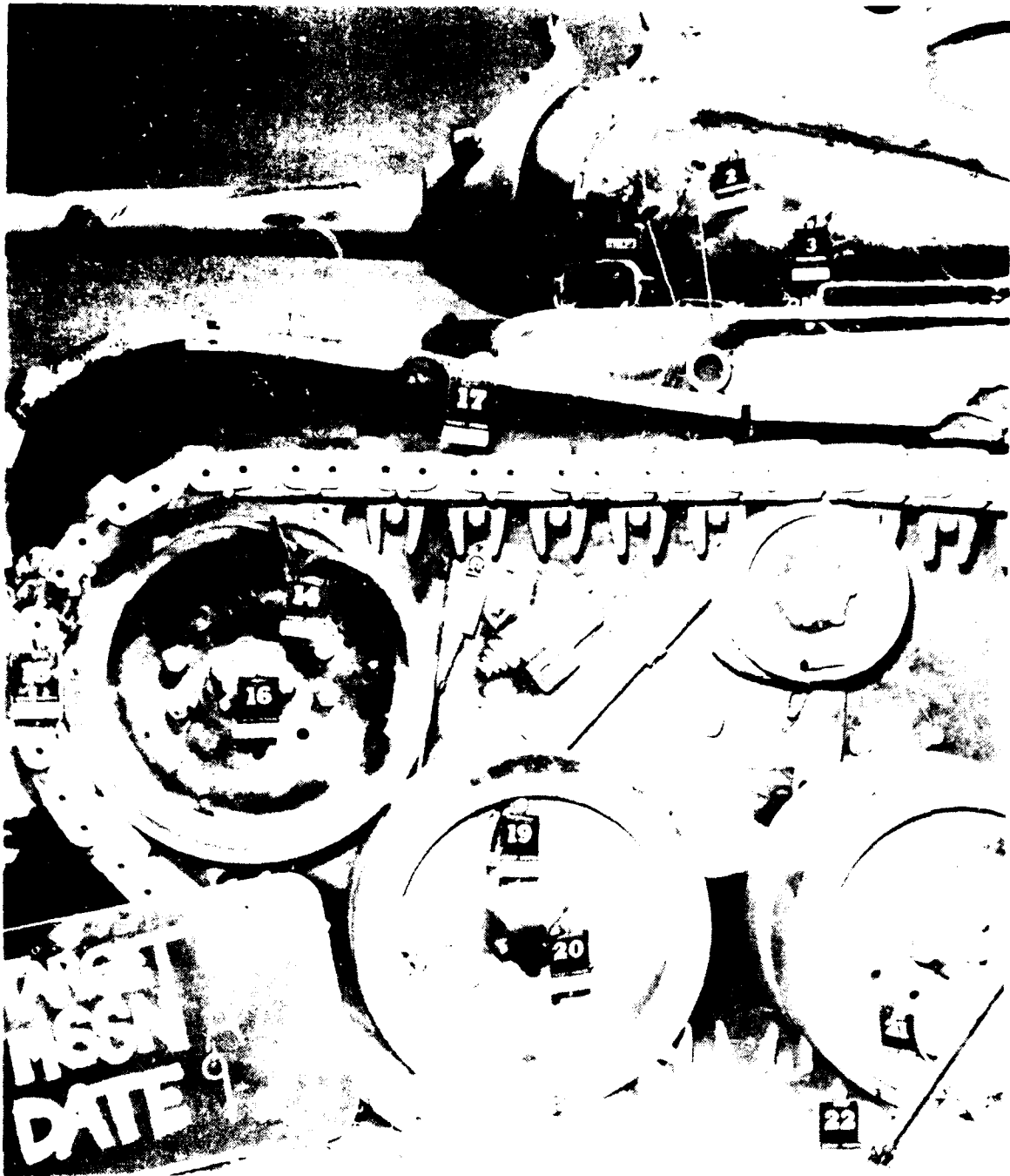
FIGURE 1. Track and Sprocket System, Tank 41.
