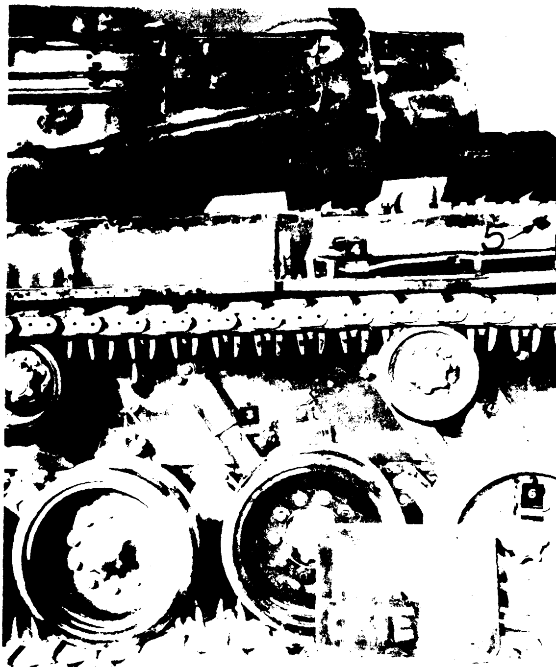
FIGURE 12. Perforation 5 Destroyed Oil Cooler Inlet Line from Transmission, Tank 10.
