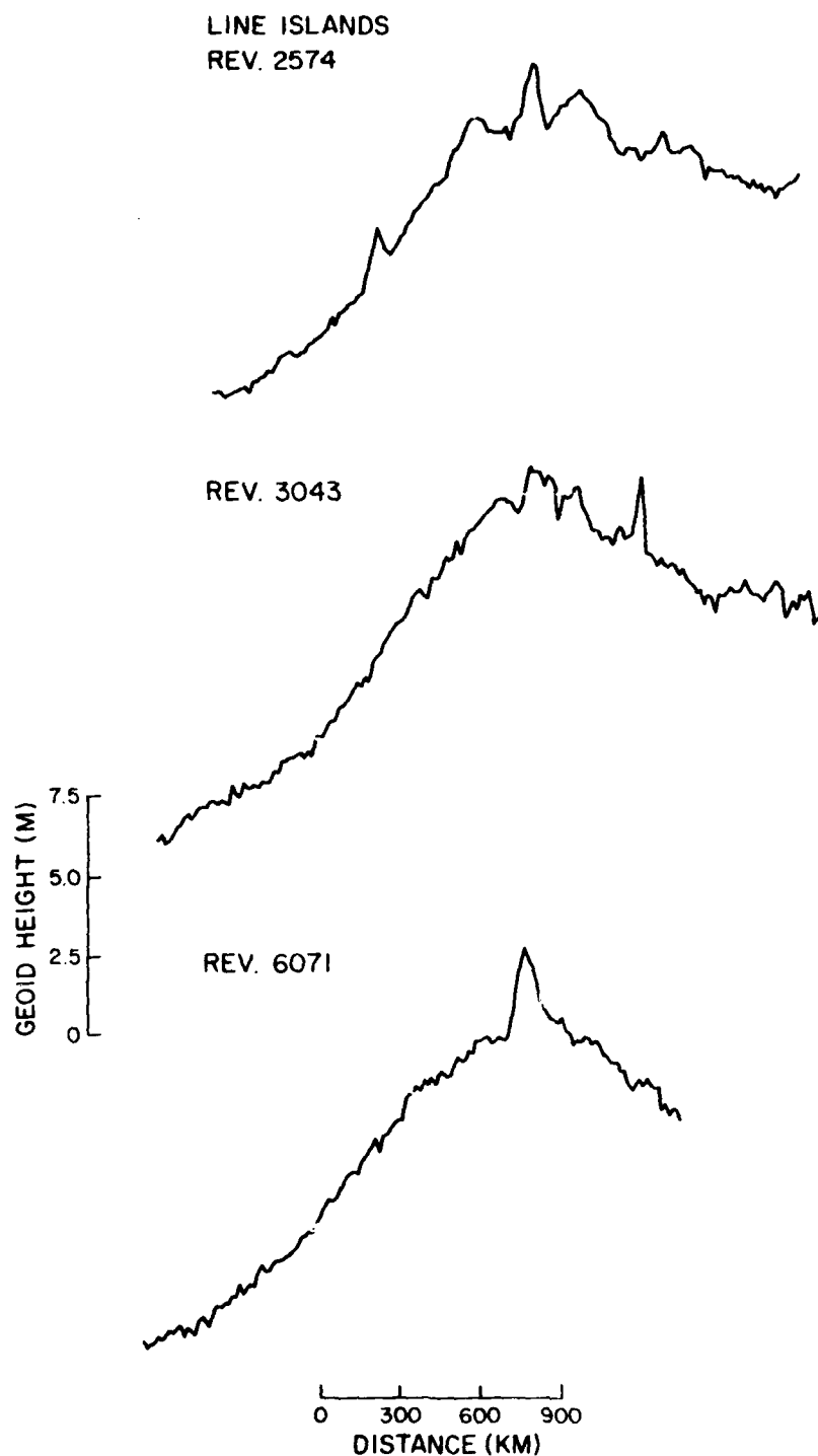
Figure 2. Three geoid height profiles crossing the Line Seamount chain. They are represented with respect to a reference geoid of degree and order calculated with GEM 10.
