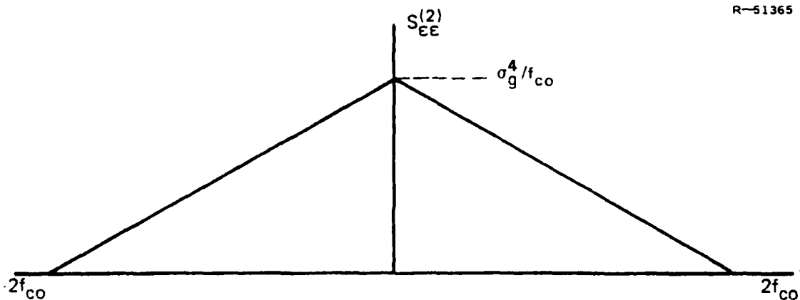
Figure A.2-1 Frequency Spectrum S_{\epsilon\epsilon}^{(2)}(f)
