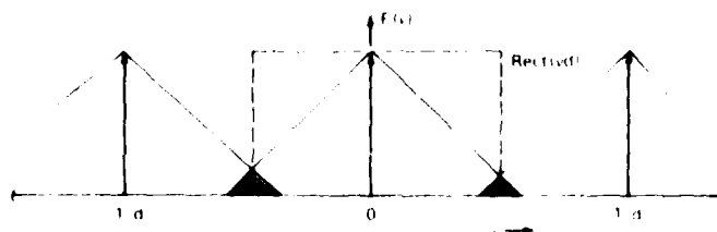
Fig. A.3 Spectrum of sampled data F(v) showing aliasing
