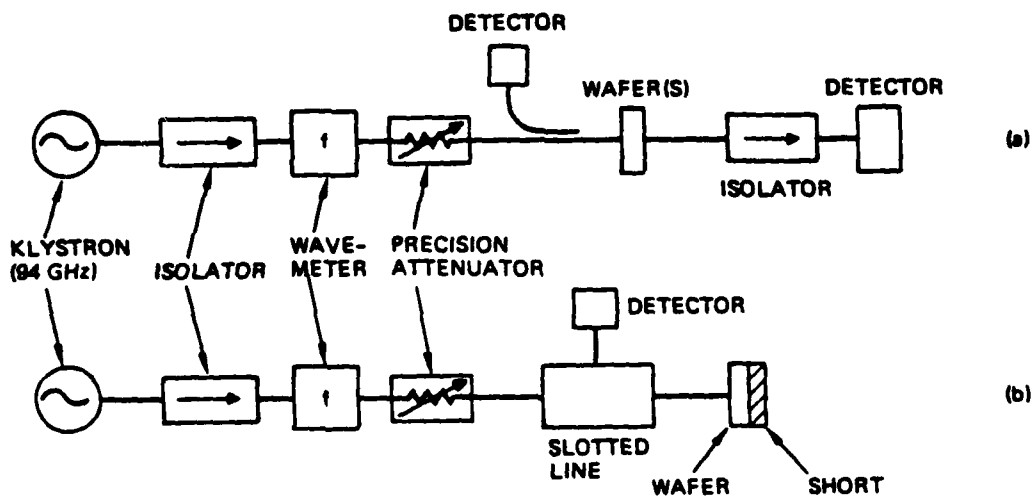
Figure II-2 Experimental arrangements used for the waveguide measurement of complex dielectric constant.
