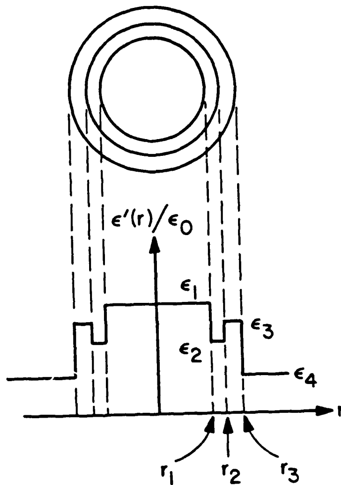
Figure V-1 Multilayer coaxial dielectric waveguide; all \epsilon_1 are real for lossless dielectrics.
