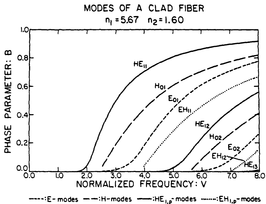
Figure IV-4 Modes of a round fiber with infinite cladding
