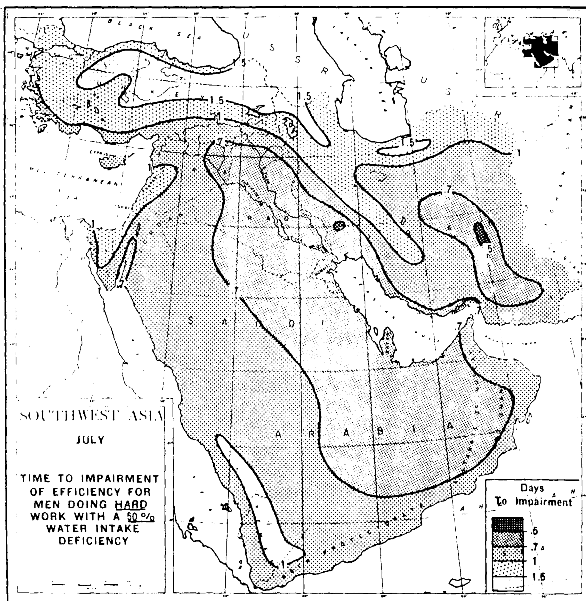
Figure C.5. Time to impairment of efficiency for men doing hard work with a 50 percent water intake deficiency (see Figure C.3 for explanation).
