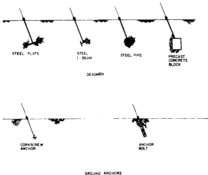
Figure 6.3. Ground anchors.
