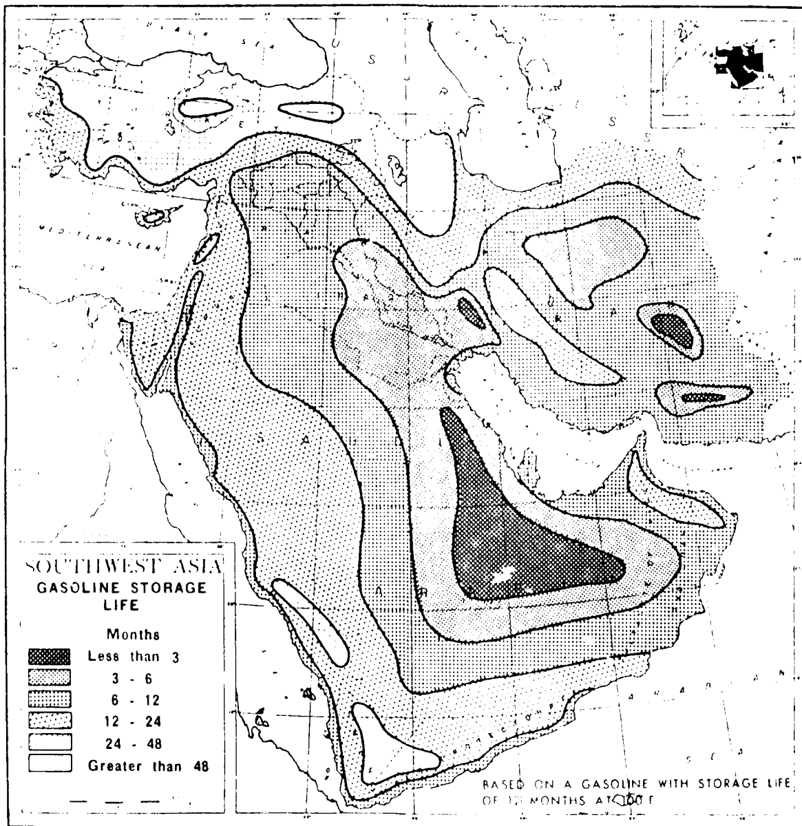
Figure 9.1. Gasoline storage life based on a gasoline with storage life of 12 months at 100°F.
