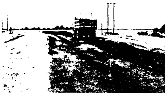
Foundation failure in soft sands. Zone IV. North Arabian Gulf
