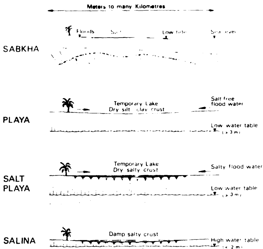
Fig. 6 Idealised cross-sections of sabkha, playa, salt playa and salina terrain. Zone IV. (see also Table 6)
