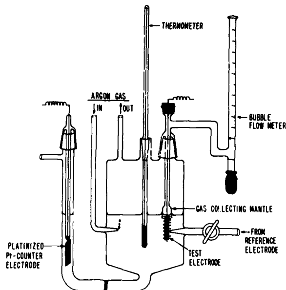
Fig. 1. Glass vessel for polarization and H_2 release measurements
