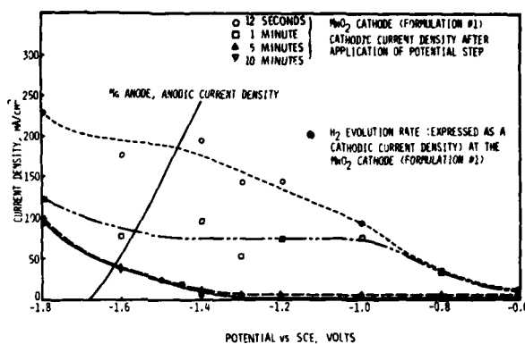
Fig. 5. Polarization behavior of fully immersed Mg anodes and MnO_2 cathodes [formulation (i)] in saturated NaCl solution.
