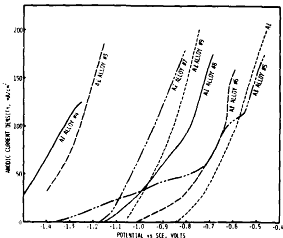
Fig. 3. Anodic polarization curves for several pure metals and aluminum alloys in saturated NaCl solution at 25°C. The curves were obtained after reversing the linear potential sweeps of Fig. 1.
