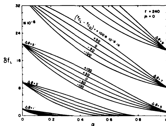
Fig. 5. Petal plots of peak-to-peak frequency deviation plotted against load capacitance parameter \alpha for odd values of crystal angle \Delta\theta .
