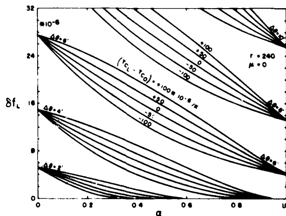
Fig. 6. Petal plots of peak-to-peak frequency deviation plotted against load capacitance parameter \alpha for even values of crystal angle \Delta\theta .
