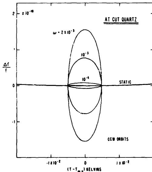
Fig. 7. Elliptical hysteresis orbits for sinusoidal temperature cycling. Temperature sweep range 5 millikelvins. This figure is drawn for \tilde{a} = -2.27 \times 10^{-7} \text{ s/K}^2 . Orbital periods are 3142, 6283, and 62832 s, corresponding to \omega = 2 \times 10^{-3} , 10^{-3} , and 10^{-4} , respectively.
