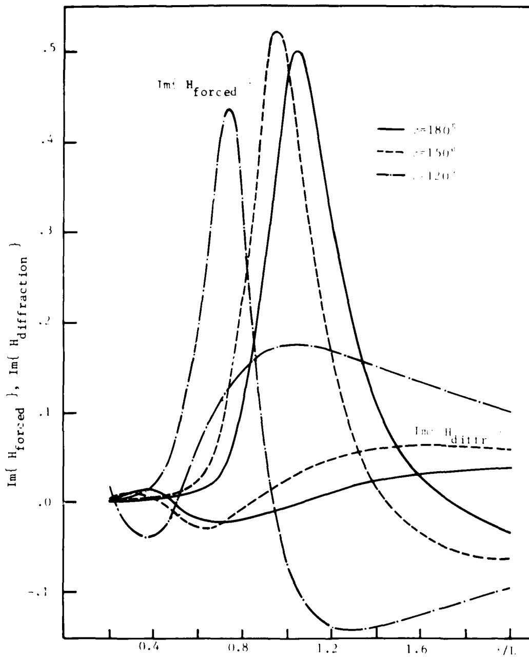
Figure 12 - The Contribution of Forced Motion and Diffraction Part to \langle \Delta P_{1IB} \rangle at F_n = 0.194
