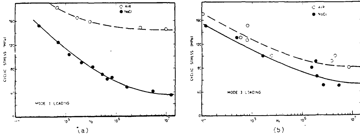
Figure 2. The effect of loading mode on fatigue resistance of 7075-T6 in 0.5 N NaCl solution. These data show that loading in shear has little effect on corrosion fatigue susceptibility when compared with tensile loading. The slight decrease in resistance which is observed in Mode III loading can probably be explained by the non-isotropic nature of the alloy.
