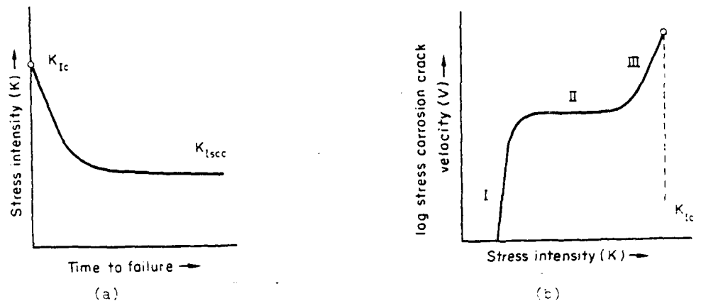
Figure 1. a) Schematic diagram of stress intensity factor ( K ) versus time to failure in a stress corrosion environment at K . Below K_{Isc} failure should not be observed. This type of data is also reported as stress versus K_{Isc} time to failure for smooth specimens, and a threshold stress level is then determined. b) Schematic diagram of crack velocity versus stress intensity factor for an alloy susceptible to SCC. K_{Isc} is often described by the intersection of stage I cracking with the K axis. Stage III cracking is not always observed and K_{Ic} is the fracture toughness of the alloy in the absence of environment.
