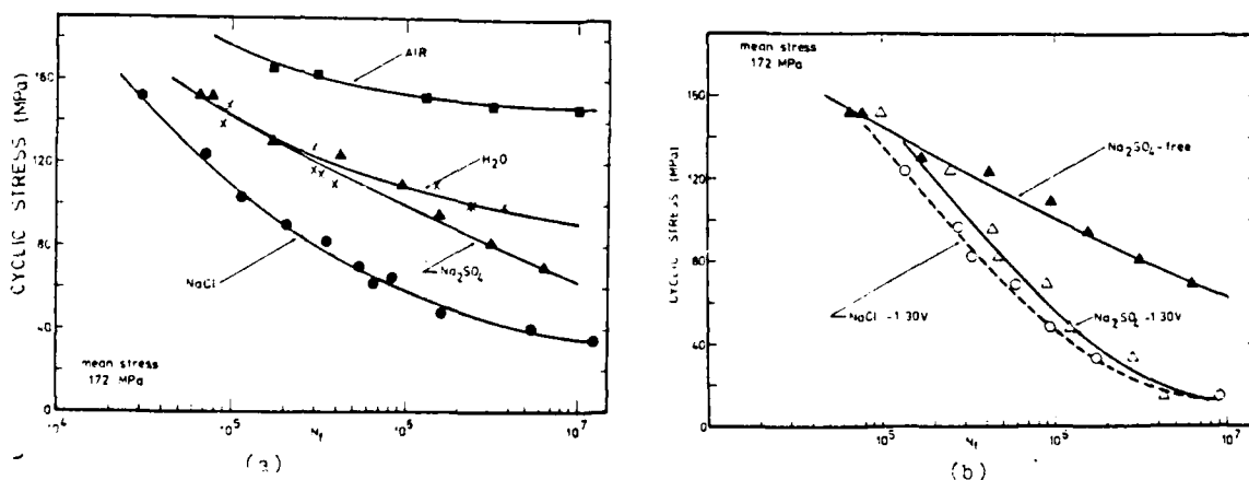
Figure 7. (a) Fatigue behavior of 7075-T6 exposed to air, \text{H}_2\text{O} and 0.5 M \text{Na}_2\text{SO}_4 and 0.5 M NaCl. \text{H}_2\text{O} and \text{Na}_2\text{SO}_4 solutions show similar behavior (see Figure 2).
