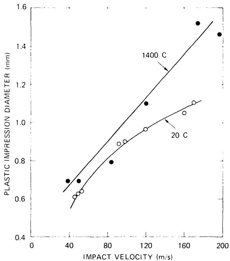
FIGURE 2 PLASTIC IMPRESSION DIAMETER VERSUS IMPACT VELOCITY FOR HP Si 3 N 4 AT ROOM TEMPERATURE AND 1400 C (2.4-mm-dia. tungsten carbide spheres)
